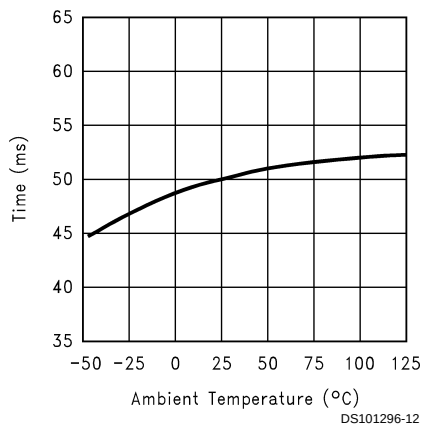
Watchdog and Reset Delay Time vs Temperature
