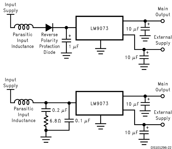
Figure 7. Input Bypassing
