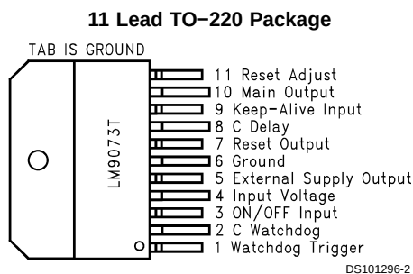
Top View Order Number LM9073T See NS Package Number TA11B
