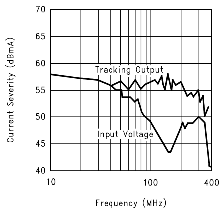
BCI Susceptibility, Modulation 2 (CW) (1kHz, 80% AM Modulation)
