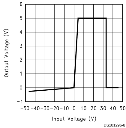
Output Voltages at Input Voltage Extremes
