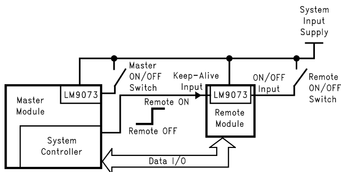
Figure 4. Remote ON/OFF Control
