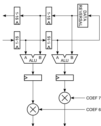
EVEN-TAP MODE
