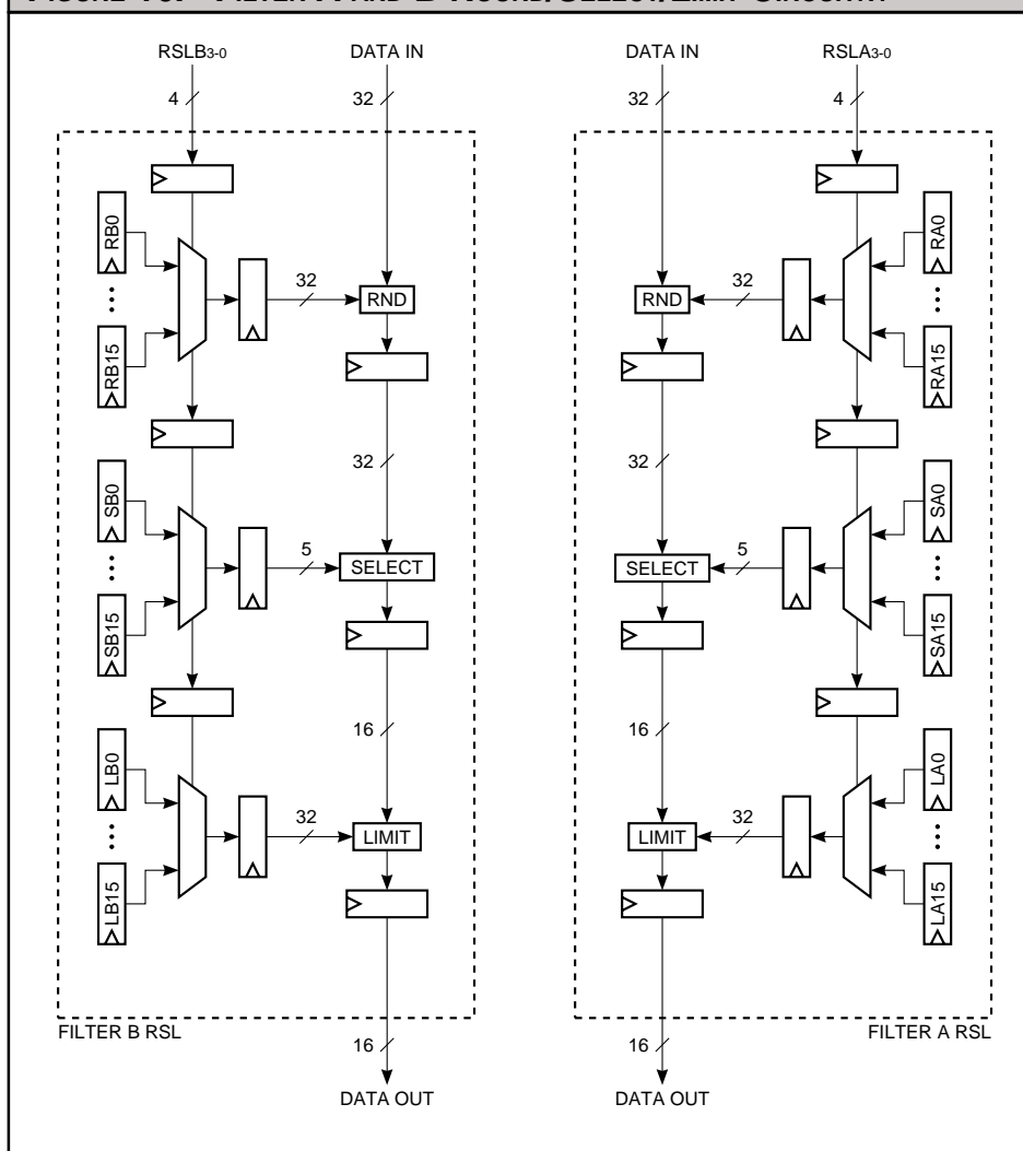
FIGURE 16. FILTER A AND B ROUND/SELECT/LIMIT CIRCUITRY
