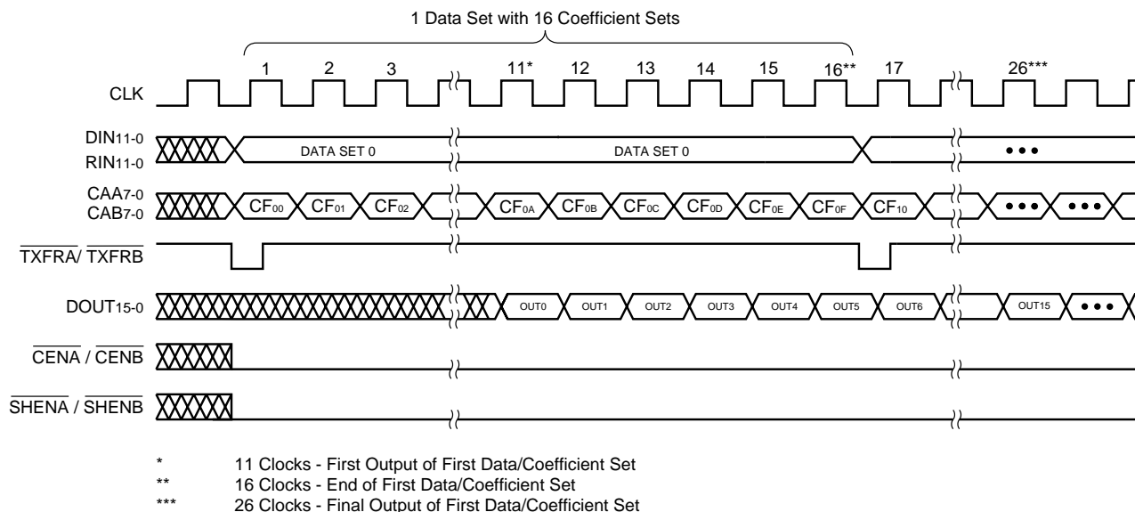
FIGURE 9. SINGLE FILTER, MATRIX MULTIPLY TIMING SEQUENCE
