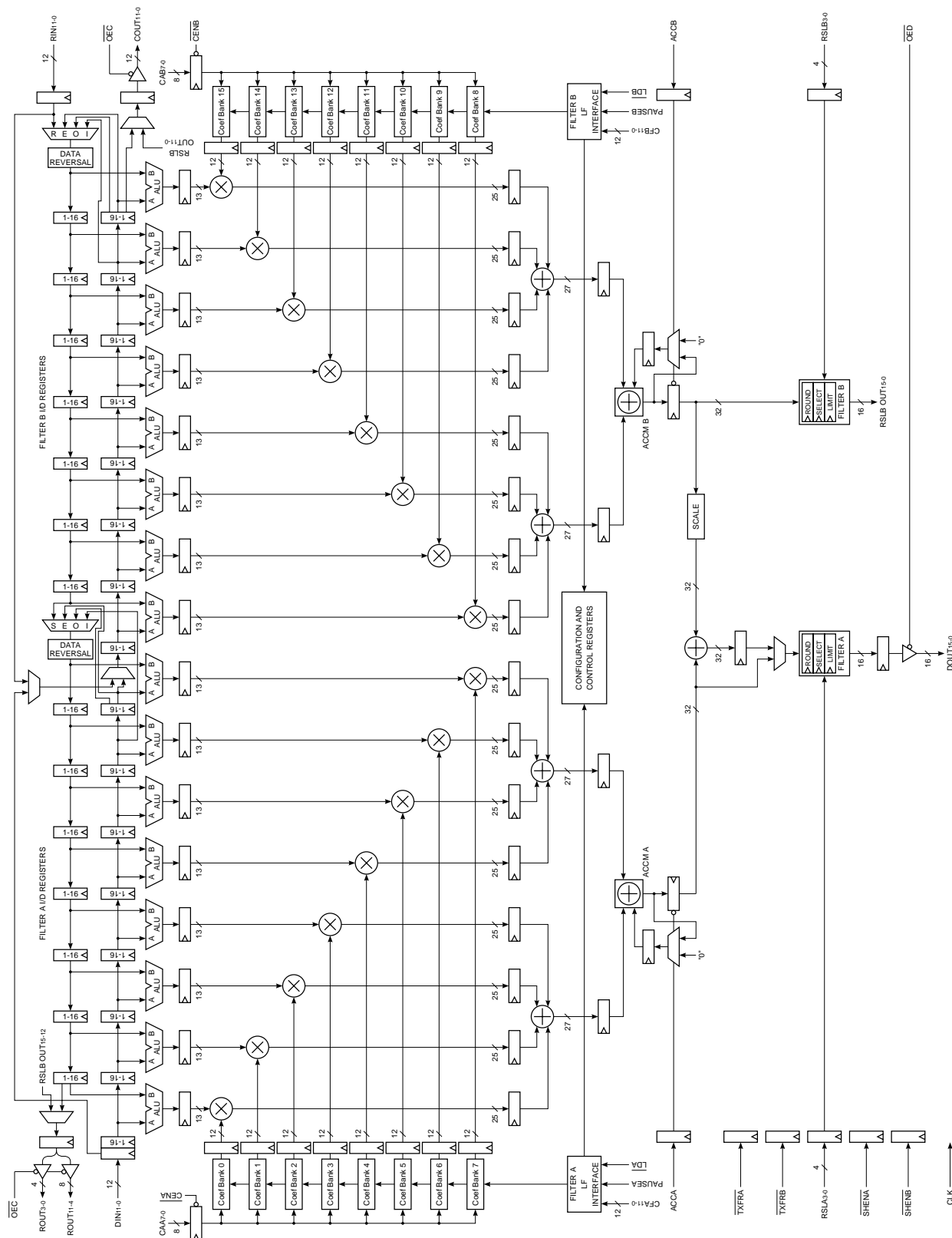
FIGURE 1. LF3320 FUNCTIONAL BLOCK DIAGRAM
