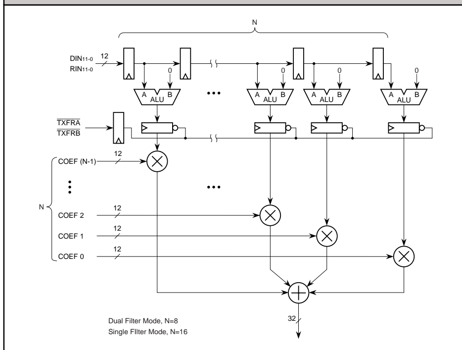
FIGURE 6. MATRIX-VECTOR MULTIPLY MODE
