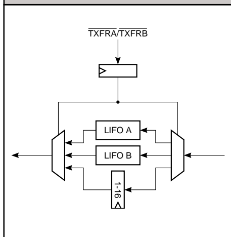
FIGURE 14. DATA REVERSAL
