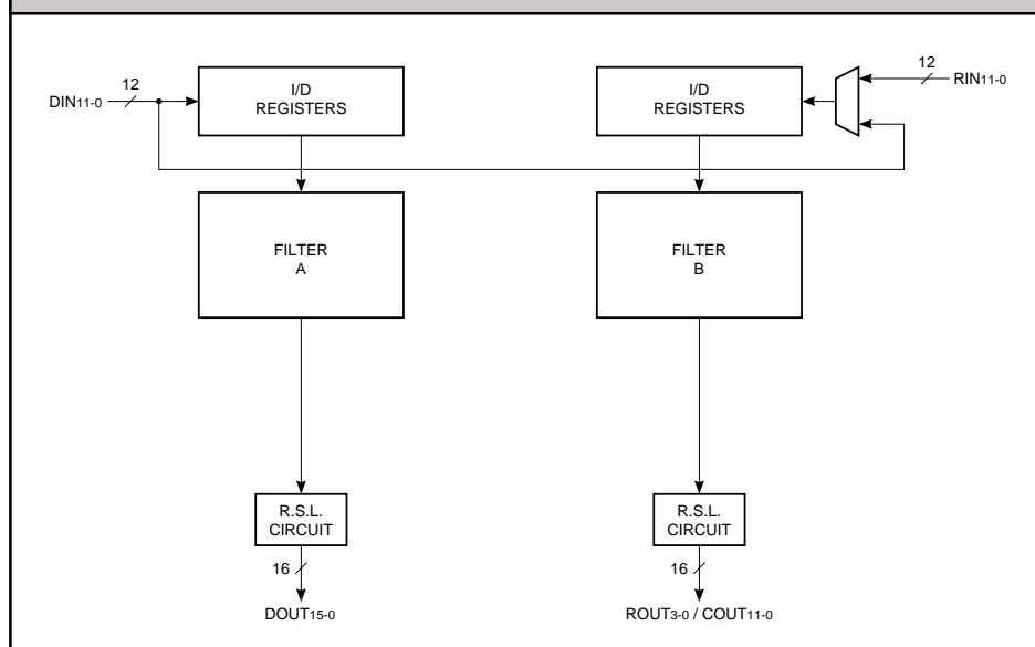
FIGURE 5. DUAL FILTER MODE
