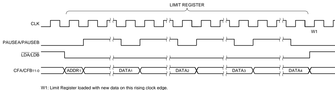
FIGURE 22. LIMIT REGISTER LOADING SEQUENCE WITH PAUSE IMPLEMENTATION
