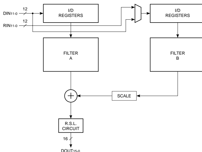
FIGURE 10. DOUBLE WIDE DATA/COEFFICIENT MODE
