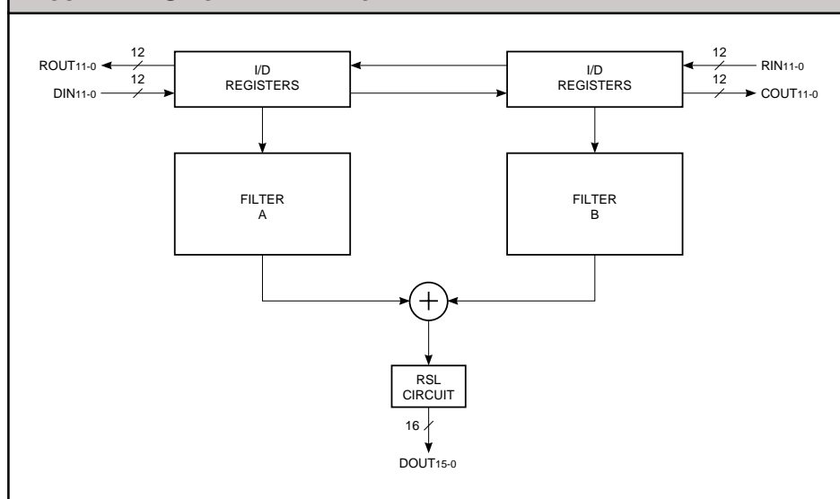
FIGURE 4. SINGLE FILTER MODE
