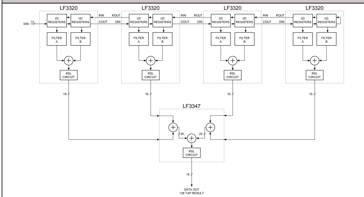
FIGURE 15. MULTIPLE LF3320s CASCADED TOGETHER
