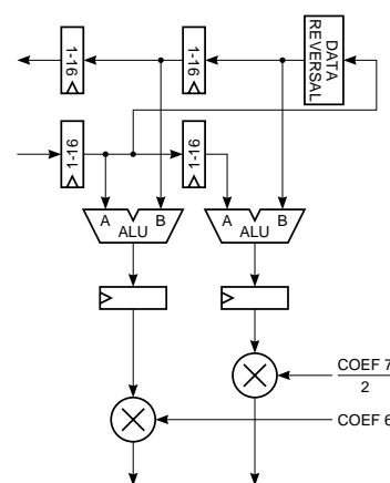
ODD-TAP INTERLEAVE MODE
