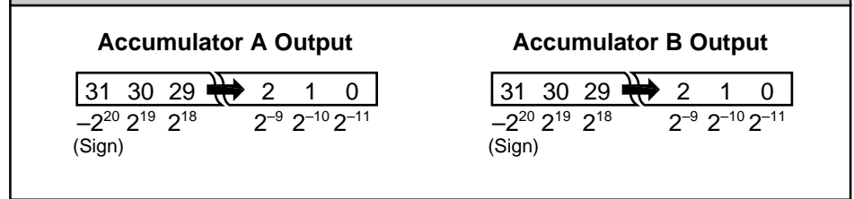
FIGURE 3. ACCUMULATOR OUTPUT FORMATS
