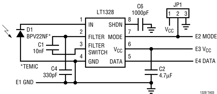
IrDA Receiver
