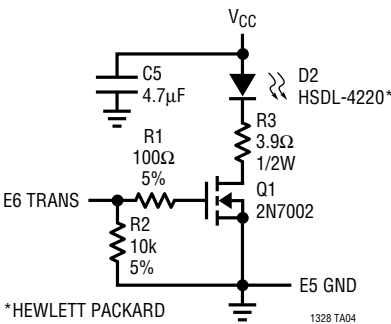
IrDA Transmitter
