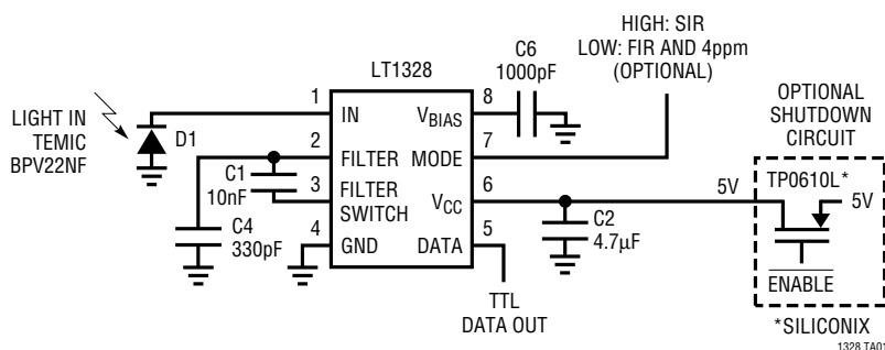
IrDA Receiver
