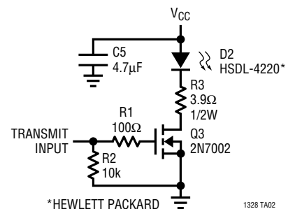
IrDA Transmitter
