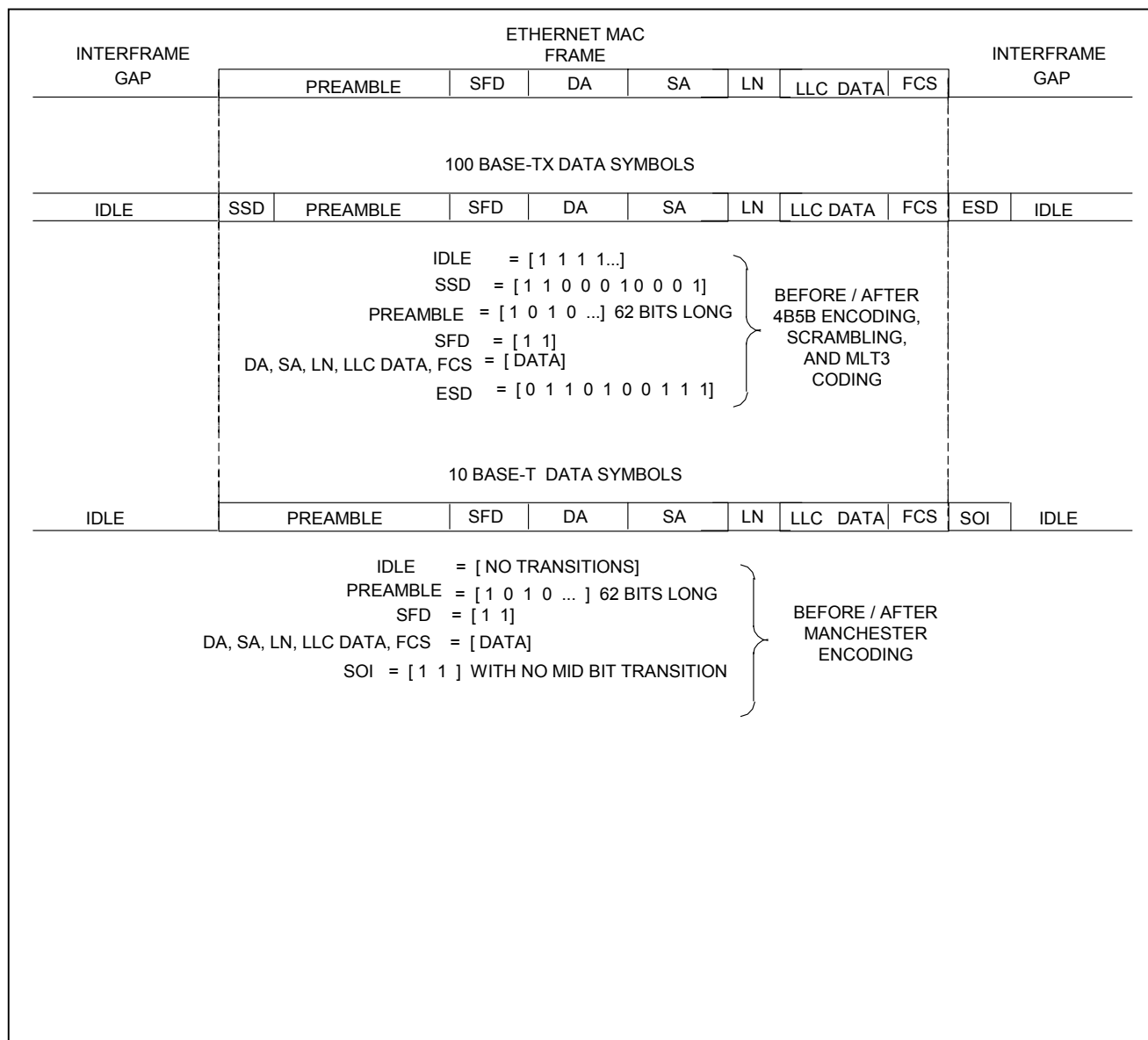
Figure 7.3 - TX/10BT Frame Format
