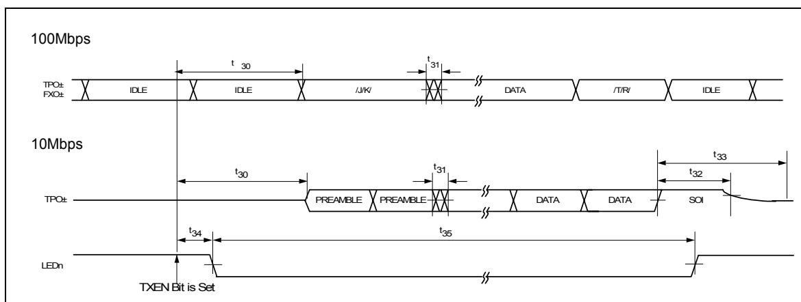
Figure 14.11 - Transmit Timing
