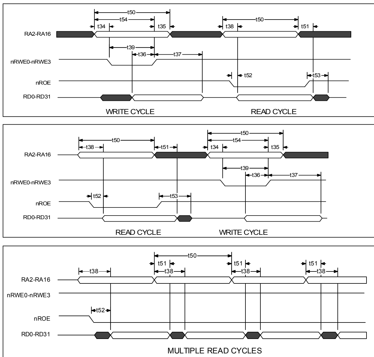
FIGURE 16 - SRAM INTERFACE
