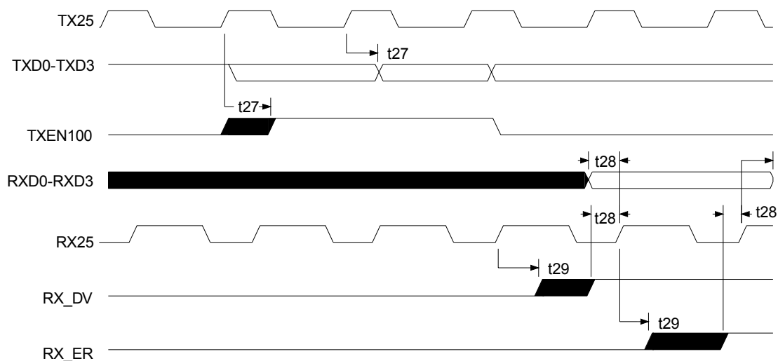
FIGURE 17 - MII INTERFACE
