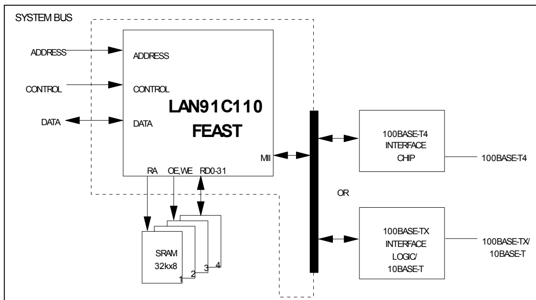
FIGURE 3 - LAN91C110 SYSTEM DIAGRAM
