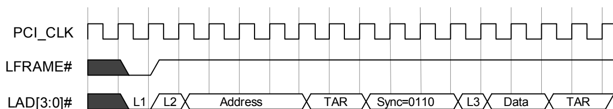
Figure 29.7 I/O Read
