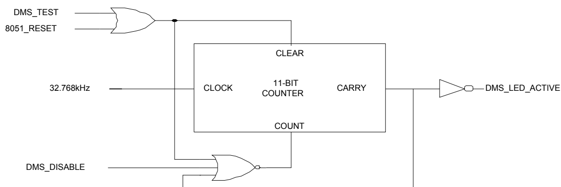
Figure 9.10 Deadman Switch Block Diagram
