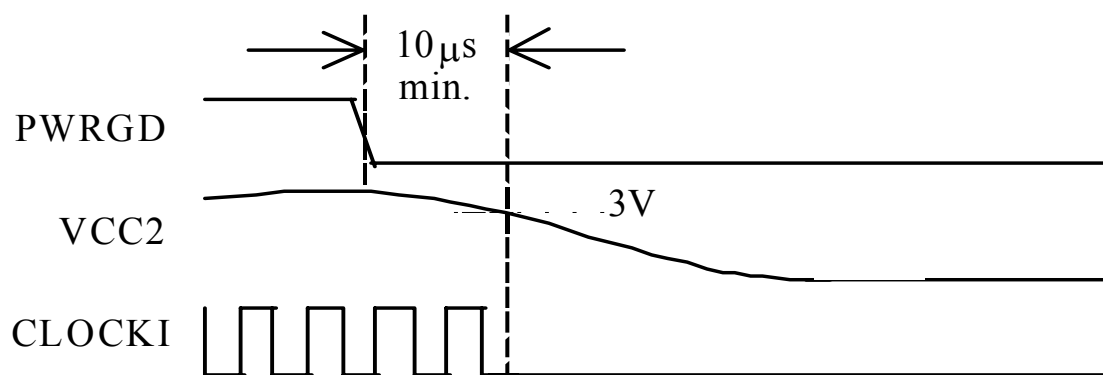
Figure 2.1 Power-Fail Event
