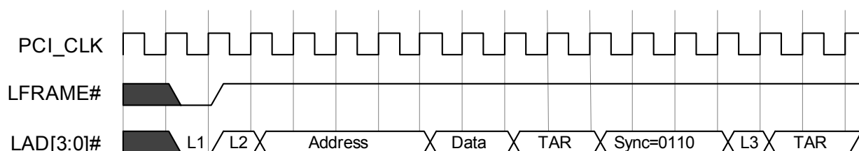
Figure 29.6 I/O Write
