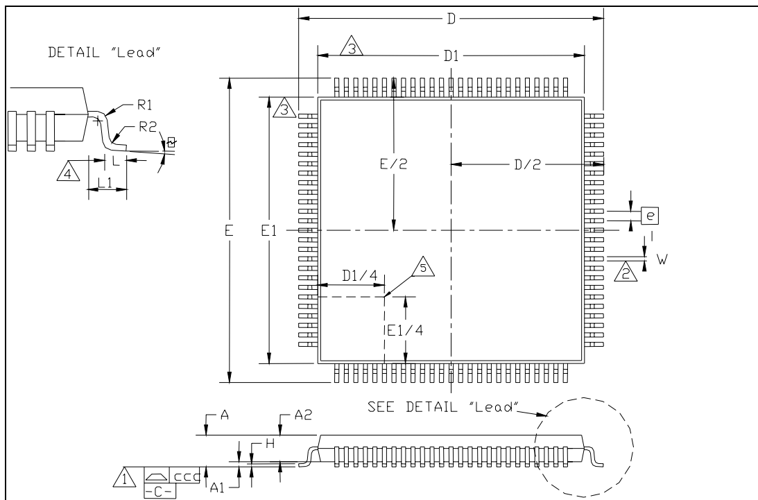
FIGURE 39 – 100 PIN STQFP, 12X12X1.4 BODY, 2.0 MM FOOTPRINT
