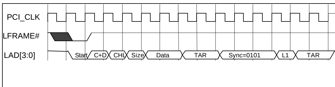
FIGURE 22 - DMA READ (FIRST BYTE)
