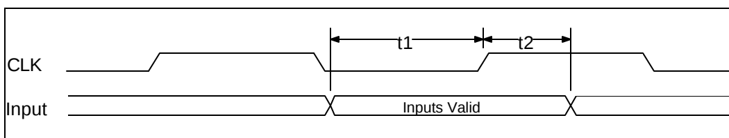
FIGURE 17 - INPUT TIMING MEASUREMENT CONDITIONS, LPC SIGNALS
