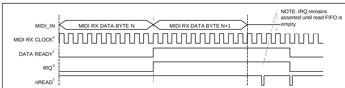
FIGURE 3 - MPU-401 INTERRUPT
