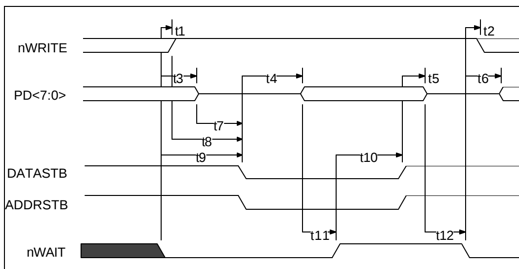
FIGURE 25 - EPP 1.9 DATA OR ADDRESS READ CYCLE
