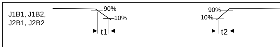
FIGURE 38 - JOYSTICK BUTTON SIGNAL
