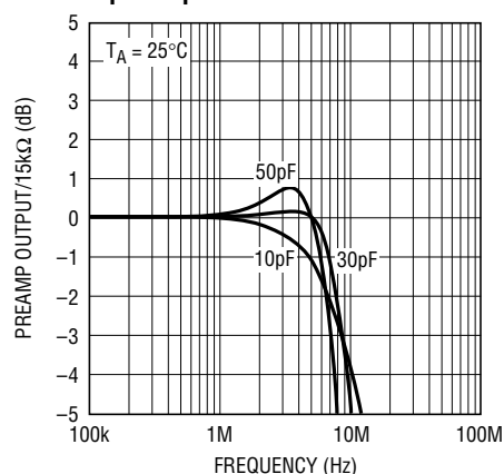
Preamp Frequency Response vs Input Capacitance
