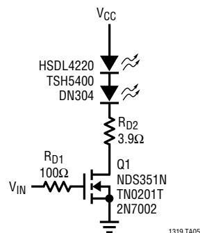
2 LED Drive Circuit for IRDA-FIR
