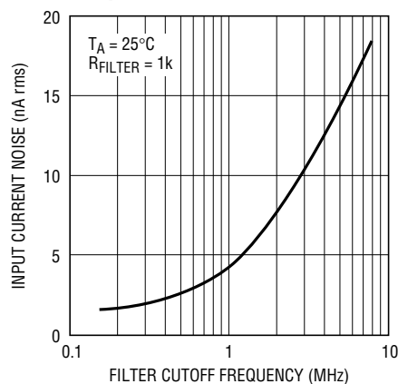
Input-Referred Noise vs Lowpass Filter on PREOUT
