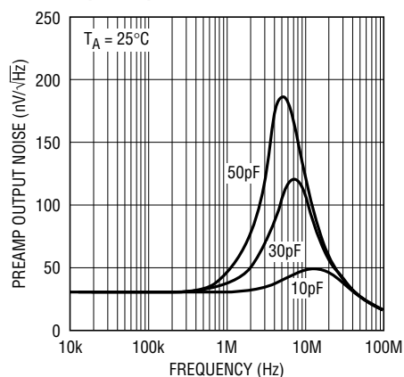
Preamp Output Noise vs Input Capacitance
