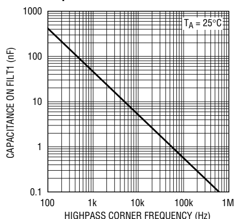
Preamp Highpass vs Capacitance on FILT1
