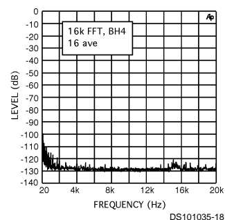
True Line Level Out Noise Floor (Analog Loopthrough)
