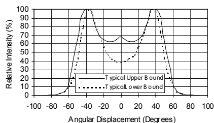
Figure 6b. Representative Spatial Radiation Pattern per Luxeon emitter for Red, Amber, Green, Cyan and Blue.
