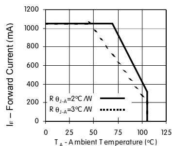
Figure 5a. Maximum Forward Current vs. Ambient Temperature. Derating based on T_{JMAX} = 120^\circ\text{C} for White, Green, Cyan and Blue18-Up.
