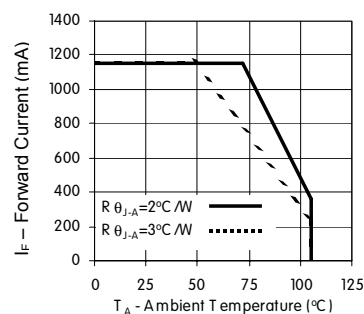
Figure 5b. Maximum Forward Current vs. Ambient Temperature. Derating based on T_{JMAX} = 120^\circ\text{C} for Red and Amber 18-Up.
