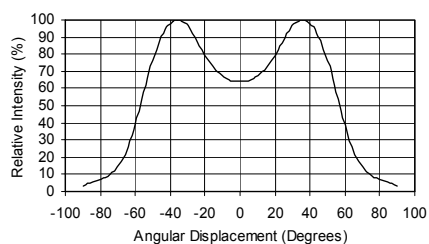
Figure 6a. Representative Spatial Radiation Pattern per Luxeon emitter, white.
