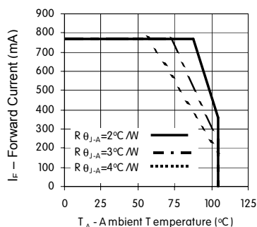
Figure 5b. Maximum Forward Current vs. Ambient Temperature. Derating based on T_{JMAX} = 120^\circ\text{C} for Red and Amber 12-Up.
