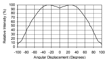
Figure 7. Representative Spatial Radiation Pattern per Luxeon emitter for Red and Amber.
