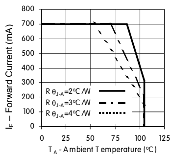
Figure 5a. Maximum Forward Current vs. Ambient Temperature. Derating based on T_{JMAX} = 120^\circ\text{C} for White, Green, Cyan and Blue12-Up.
