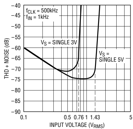
Dynamic Range THD + Noise vs Input Voltage
