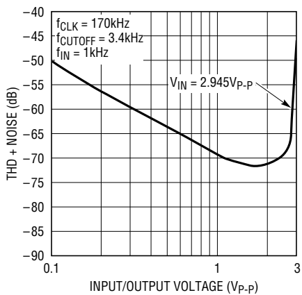
Dynamic Range THD + Noise vs Input/Output Voltage
