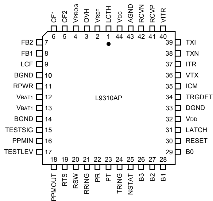
Figure 3. 44-Pin PLCC
