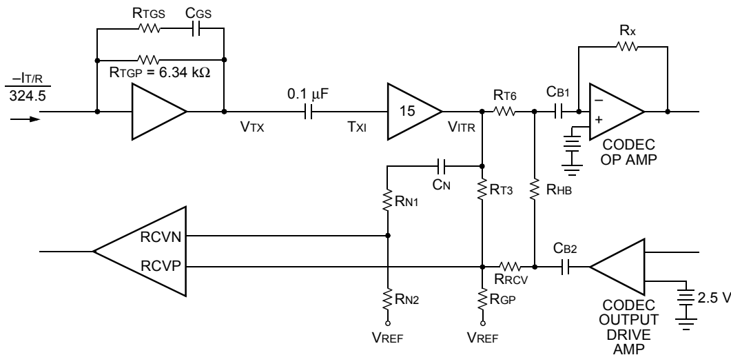
Figure 18. ac Interface Using First-Generation Codec (Including Blocking Capacitors) for Complex Termination Impedance
