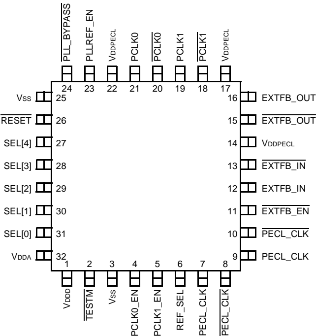
Figure 2. 32-Pin TQFP
