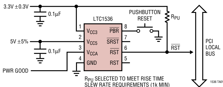
Motherboard PCI \overline{RST} Generation
