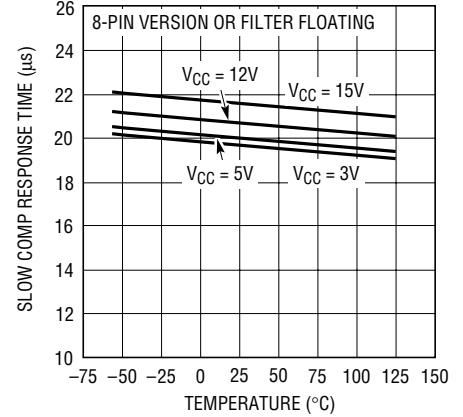
SLOW COMP Response Time vs Temperature
