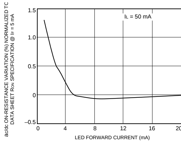
F. Variation in ON-Resistance vs. LED Current
