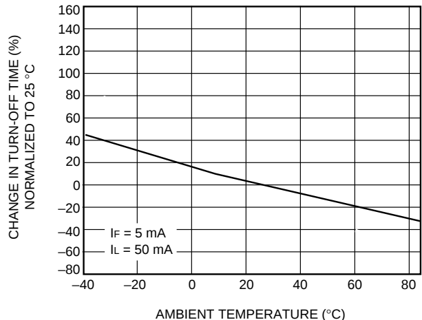
D. Turn-Off Time vs. Temperature
