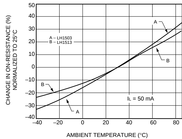
E. ON-Resistance vs. Temperature
