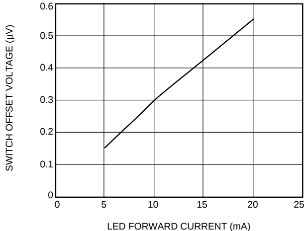
B. Switch Offset Voltage vs. LED Current
