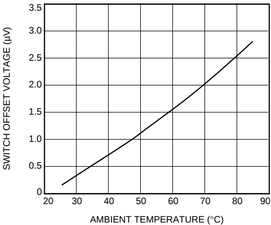
A. Switch Offset Voltage vs. Temperature
