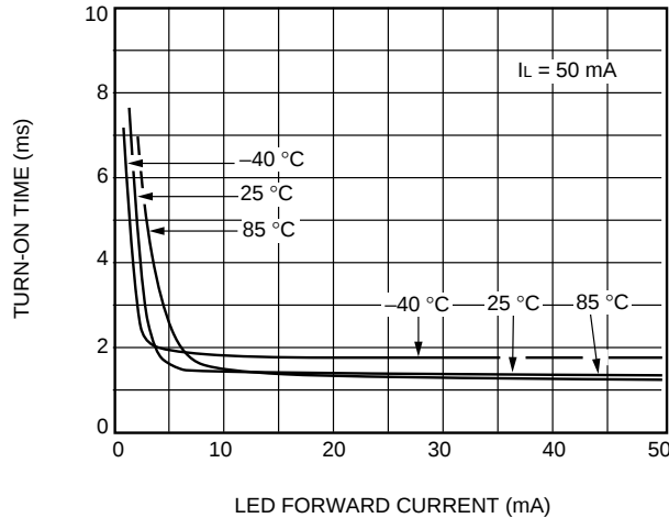
E. Turn-On Time vs. LED Current
