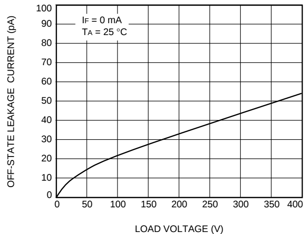
D. Leakage Current vs. Applied Voltage
