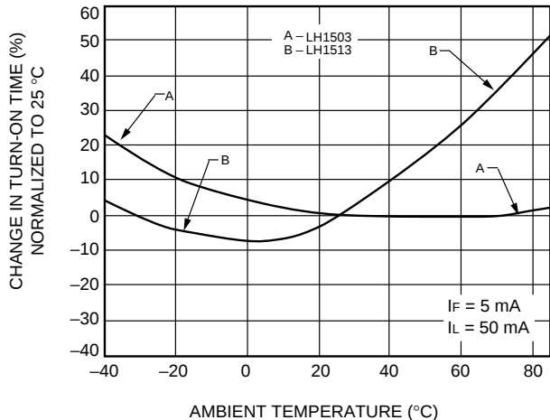
C. Turn-On Time vs. Temperature
