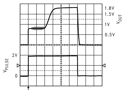
Turn-On Time
