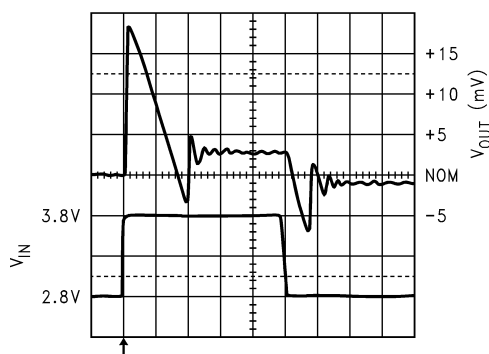
Line Transient
