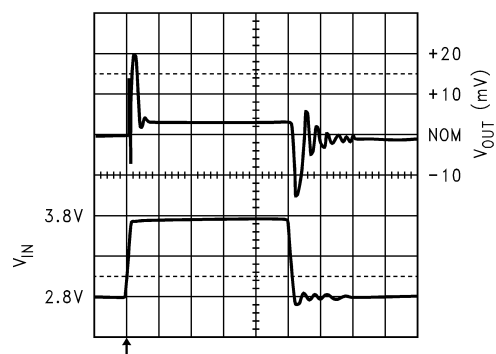
Line Transient
