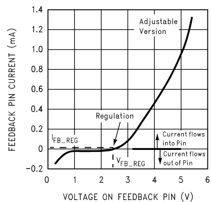
Characteristics of Feedback Pin
