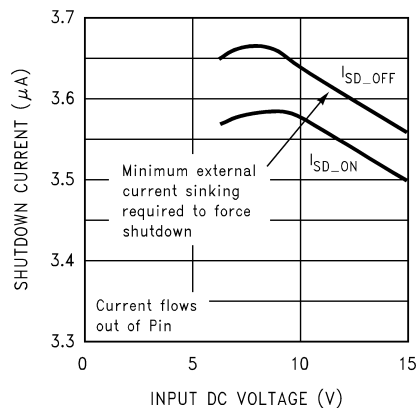
Shutdown Pin Current at Shutdown Threshold
