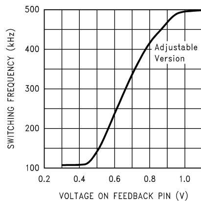
Frequency Foldback
