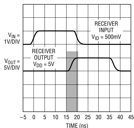
Propagation Delay Guaranteed to Fall Within Shaded Area ( \pm 3\text{ns} )
