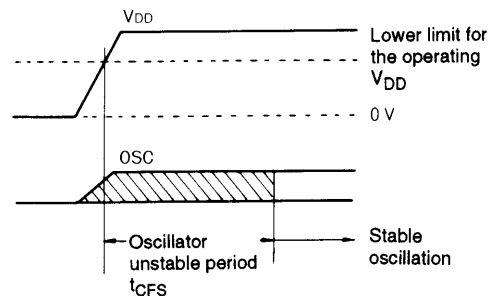
Figure 3 Oscillator Stabilization Period
