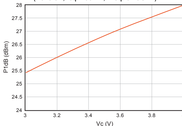
Typical P1dB vs. Supply Voltage (Vc=3.3V, Icq=100mA, Freq=5.25GHz)
