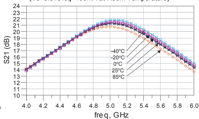
Typical Small-Signal Gain Variation Over Temperature (Vc=3.3V, Icq=100mA at Room Temperature)
