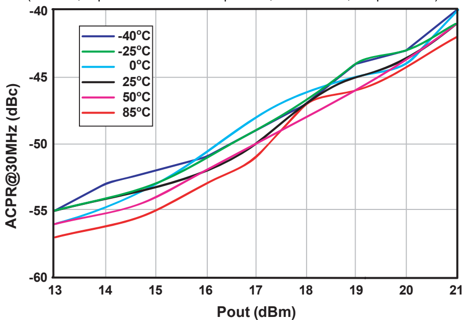
Typical ACPR Variation Over Temperature
