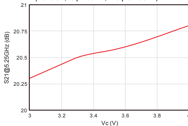
Typical Small-Signal Gain vs. Supply Voltage (Vc=3.3V, Icq=100mA, Freq=5.25GHz)
