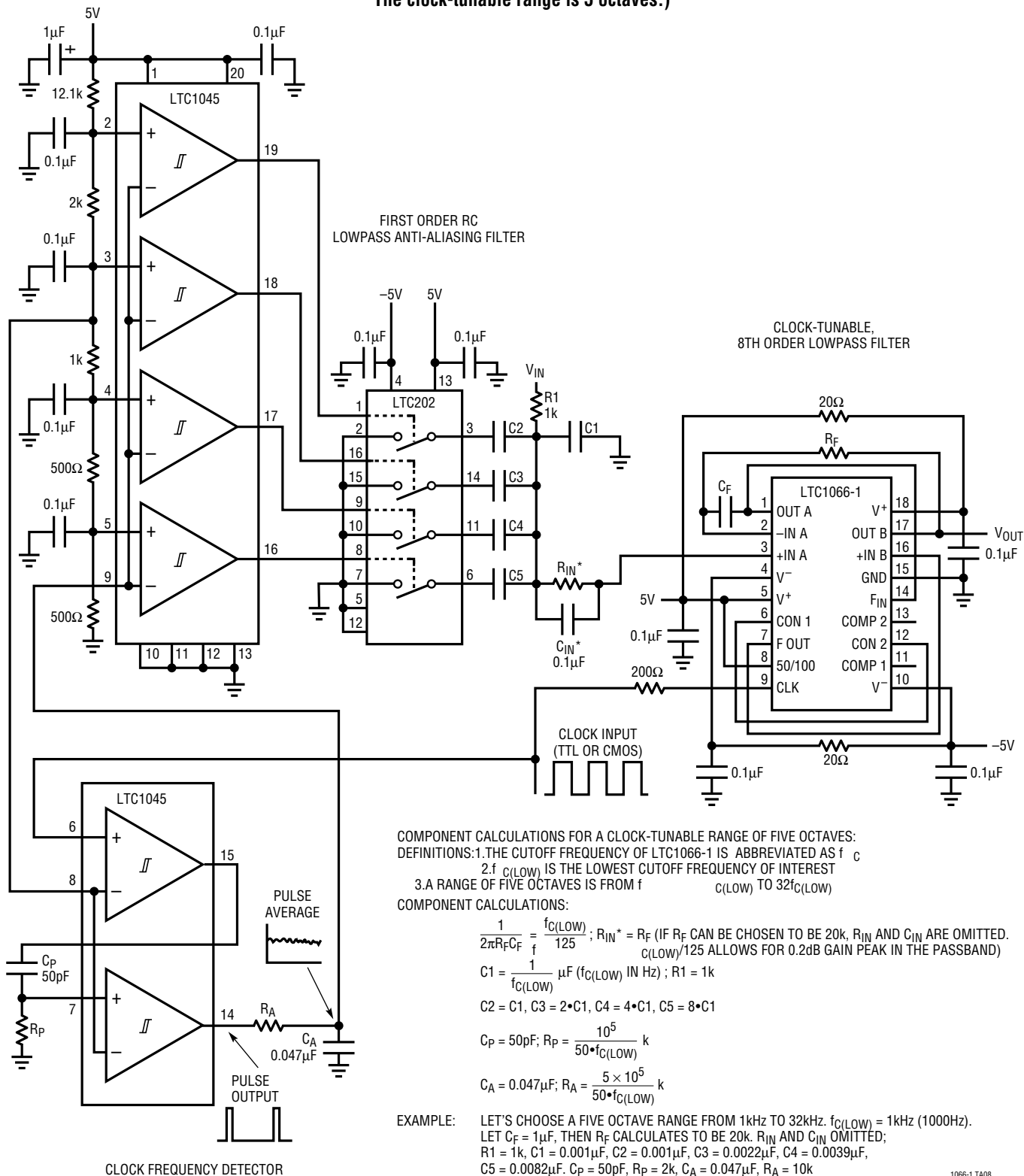
DC Accurate Clock-Tunable Lowpass Filter with Tunable Input Anti-Aliasing Filter (Circuit provides at least -20\text{dB} attenuation to input frequencies at 2f_{\text{CLK}} . The clock-tunable range is 5 octaves.)
