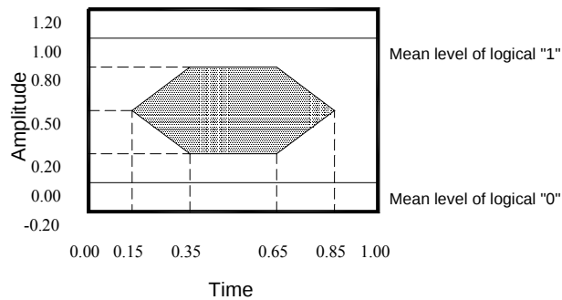
Optical Pulse Mask with Bessel Filter Specified in ITU-T G.957
