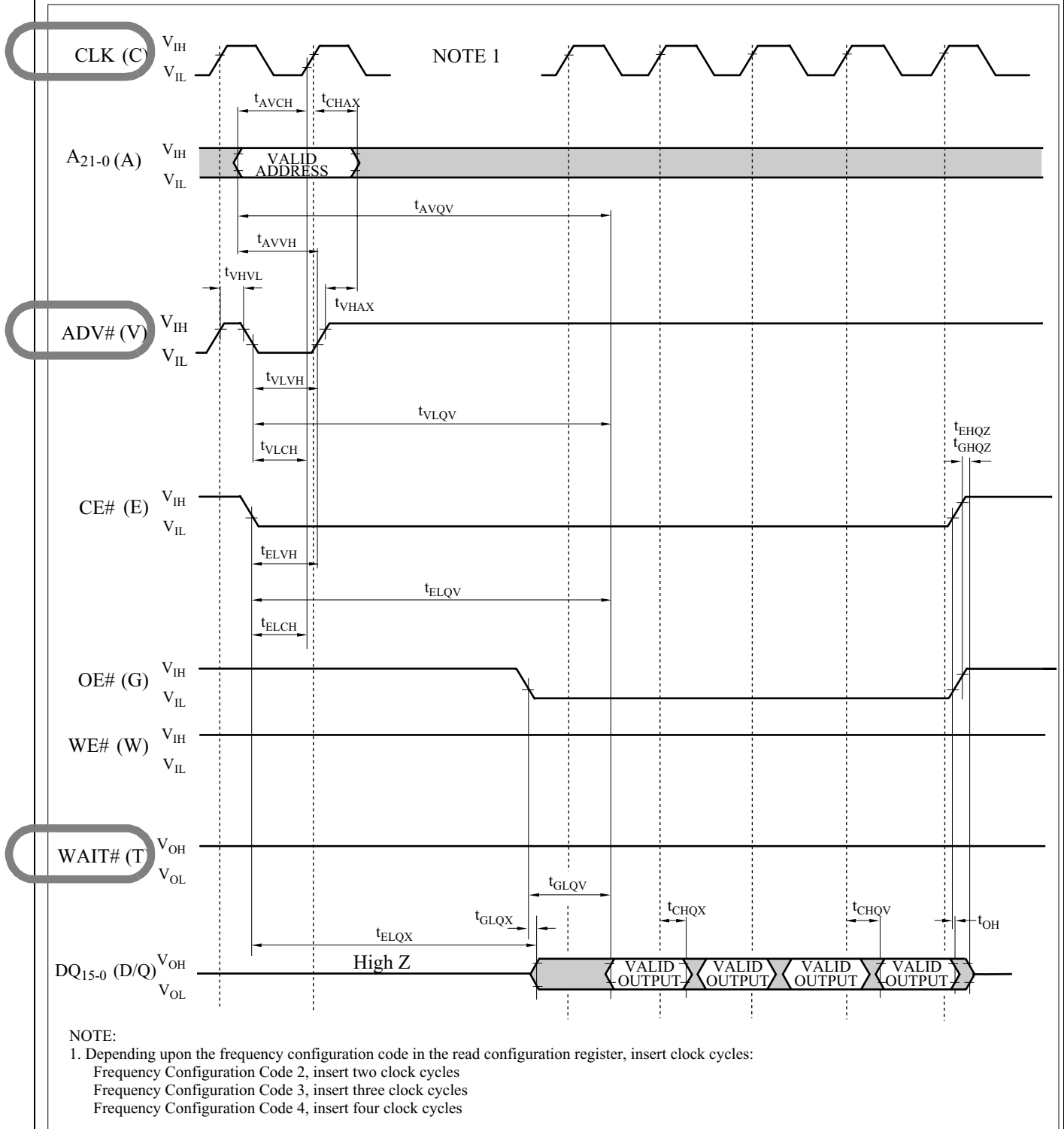
Figure 19. AC Waveform for Synchronous Burst Mode Read Operations from Main Blocks or Parameter Blocks in 4-Word Burst Mode: RCR.2-0=001 (A 21 is not used for 32M-bit device.)
