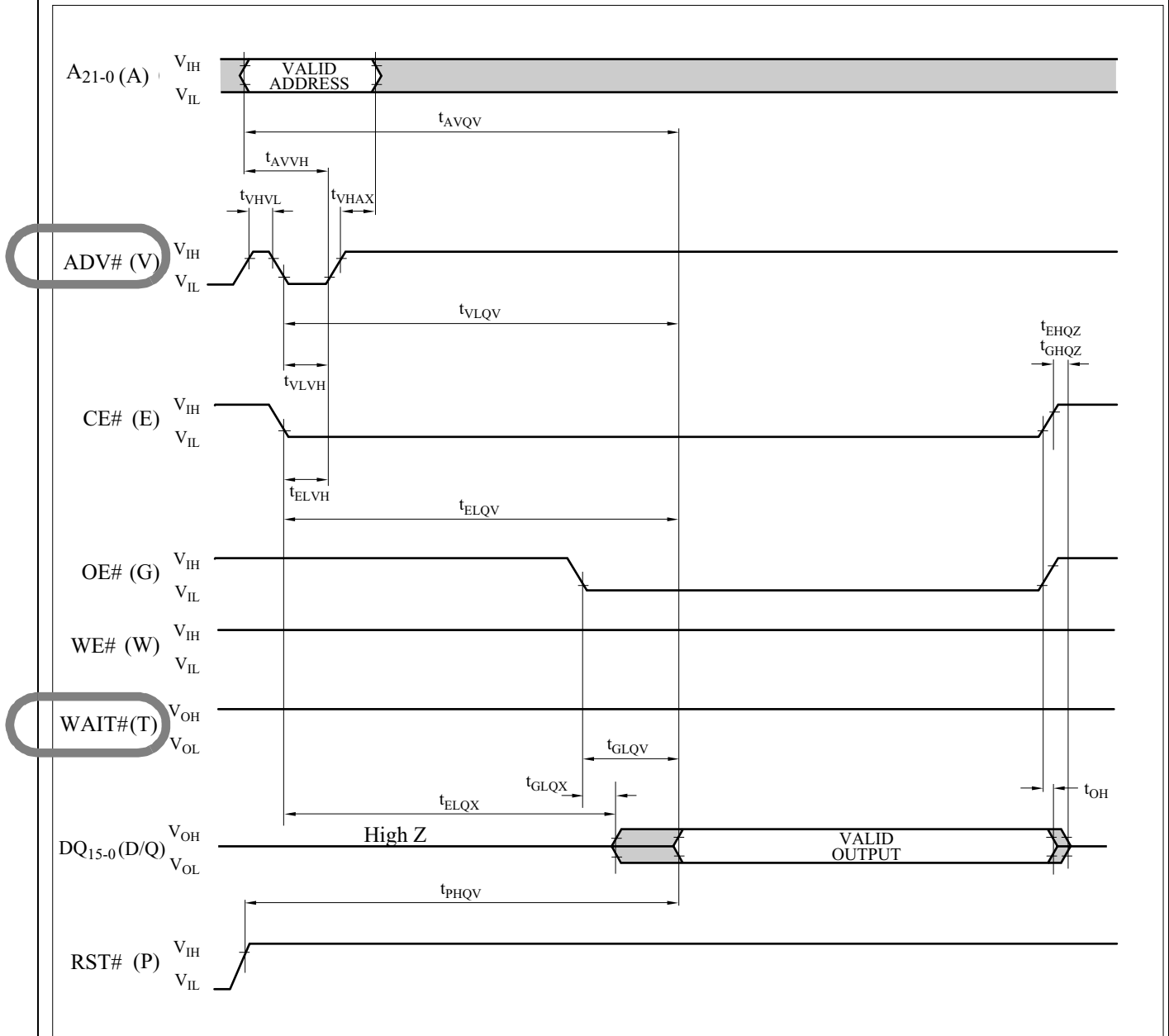
Figure 21. AC Waveform for Single Asynchronous Read Operations from Status Register, Identifier Codes, OTP Block or Query Code (A 21 is not used for 32M-bit device.)
