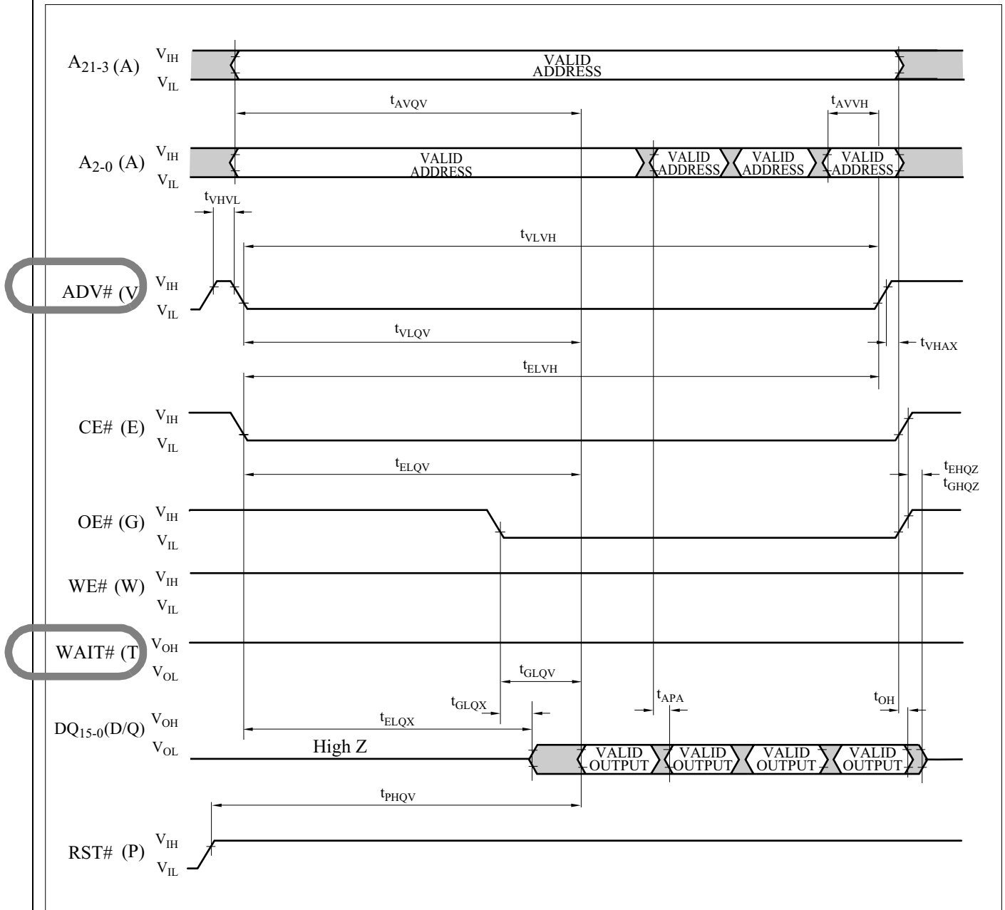
Figure 18. AC Waveform for Asynchronous Page Mode Read Operations from Main Blocks or Parameter Blocks (A 21 is not used for 32M-bit device.)
