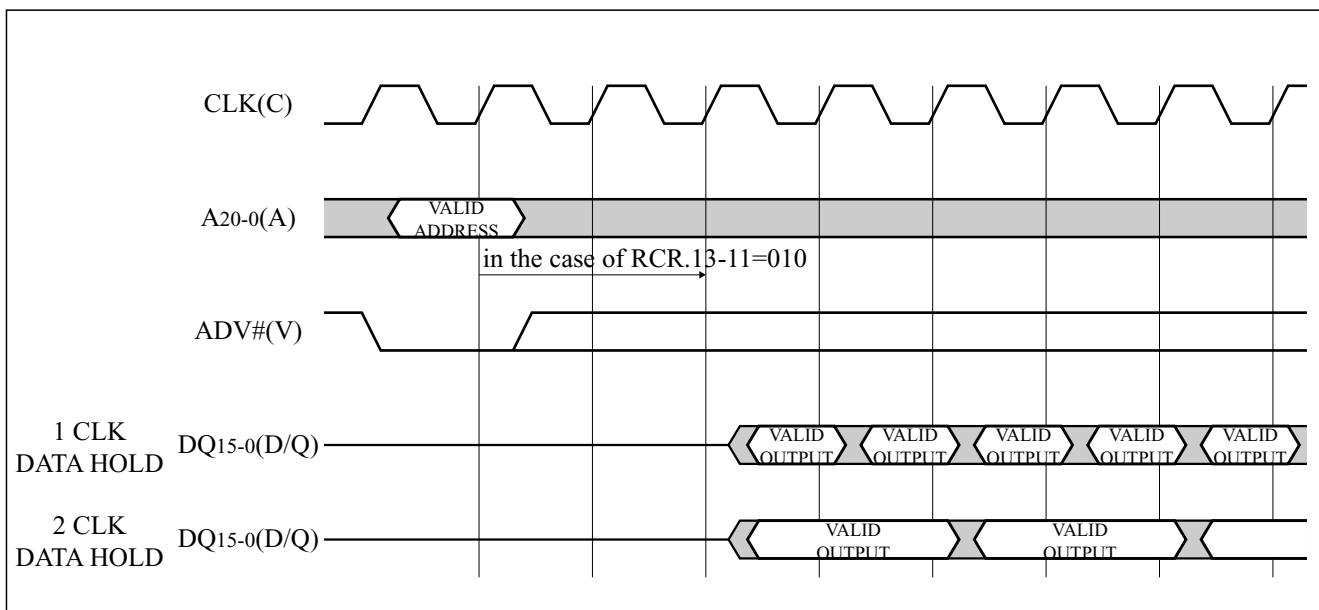
Figure 15. Output Configuration
