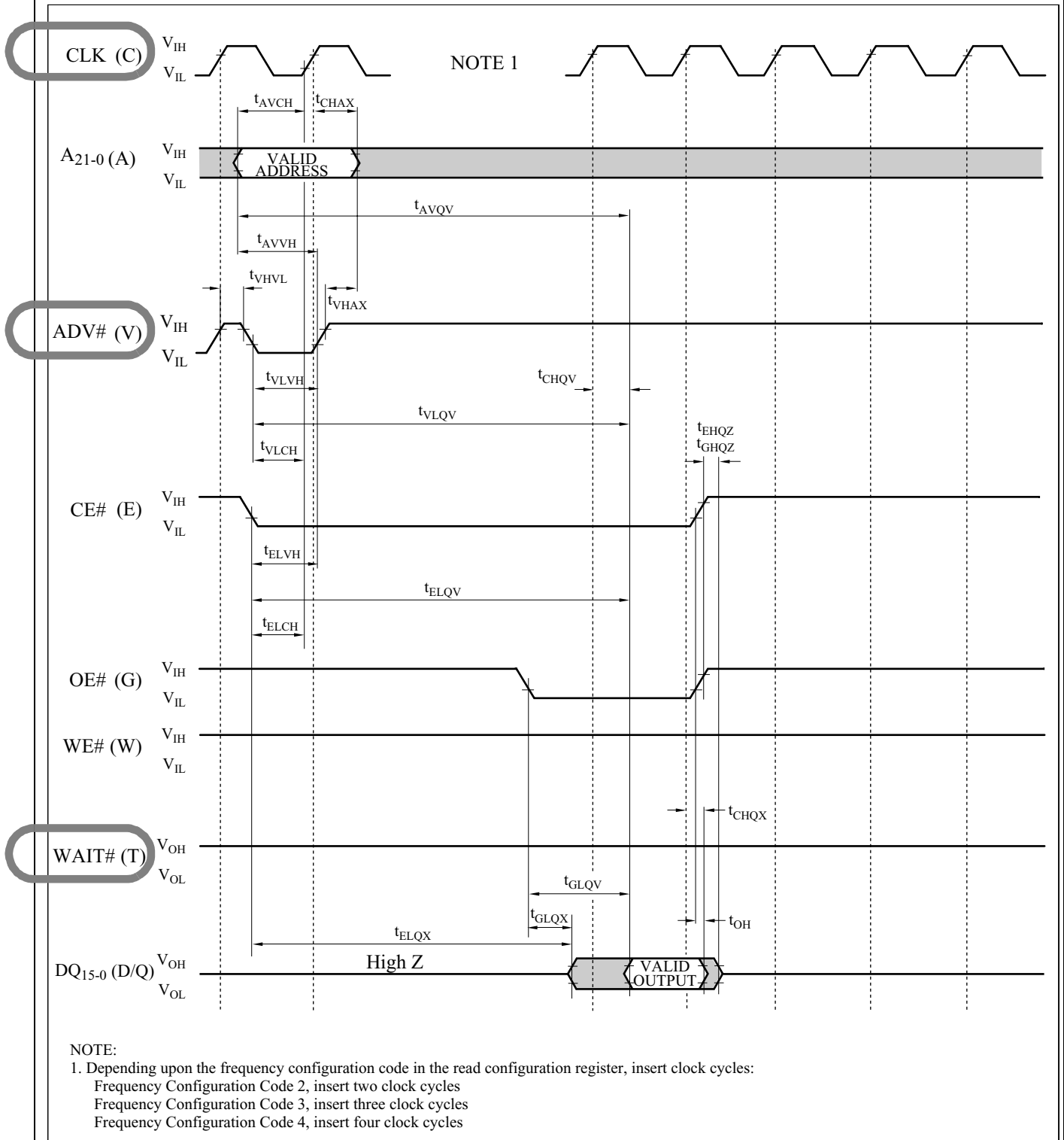
Figure 22. AC Waveform for Single Synchronous Read Operations from Status Register, Identifier Codes, OTP Block or Query Code (A 21 is not used for 32M-bit device.)
