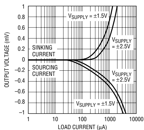
Op Amp Output Voltage vs Load Current
