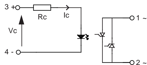
Figure 3 — LS relays
