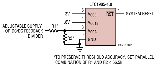
Triple Supply Monitor (3V, 1.8V and Adjustable)
