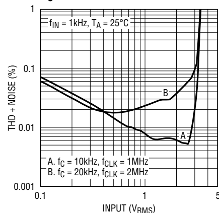
THD + Noise vs Input Voltage; V_S = \pm 5\text{V}
