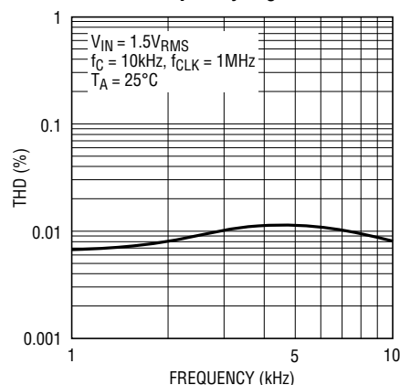
THD vs Frequency; V_S = \pm 5\text{V}
