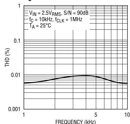
THD vs Frequency; V_S = \pm 7.5\text{V}
