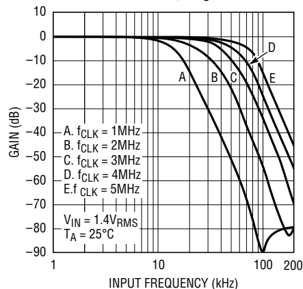
Gain vs Frequency; V_S = \pm 7.5\text{V}
