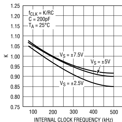
Figure 4b. f_{CIK} vs K
