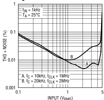
THD + Noise vs Input Voltage; V_S = \pm 7.5\text{V}
