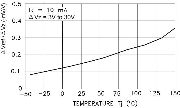
Ratio of Delta Reference Voltage to Delta Cathode Voltage VS. Junction Temperature
