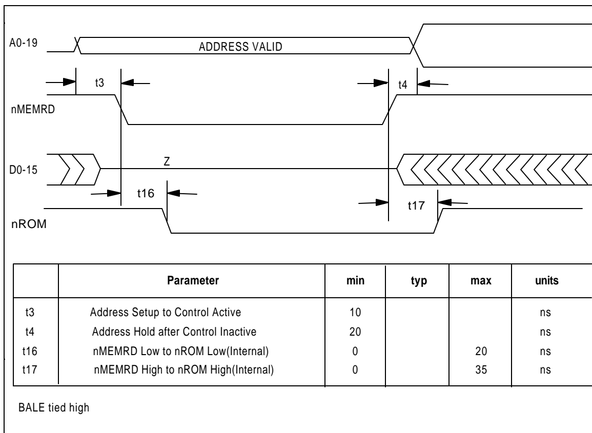
FIGURE 27 - EXTERNAL ROM READ ACCESS
