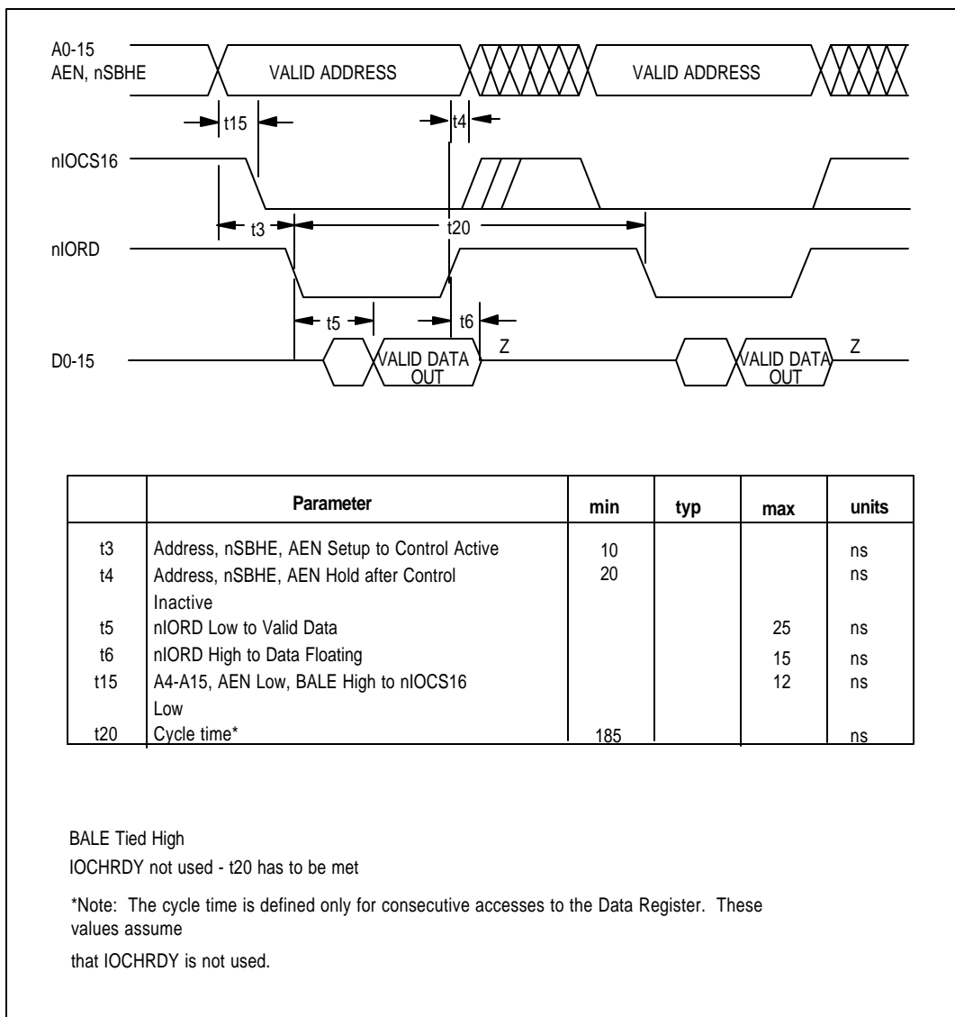
FIGURE 21 - LOCAL BUS CONSECUTIVE READ CYCLES
