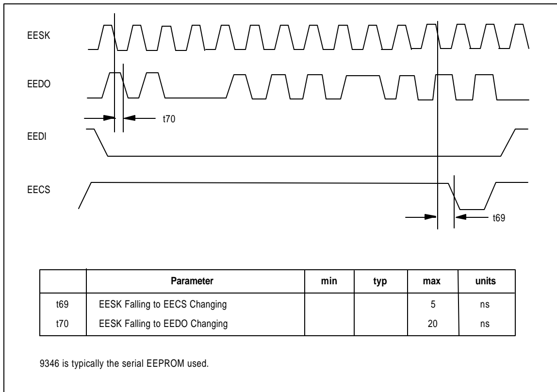
FIGURE 31 - EEPROM WRITE
