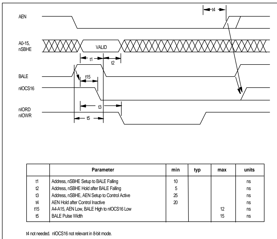
FIGURE 28 - LOCAL BUS REGISTER ACCESS WHEN USING BALE
