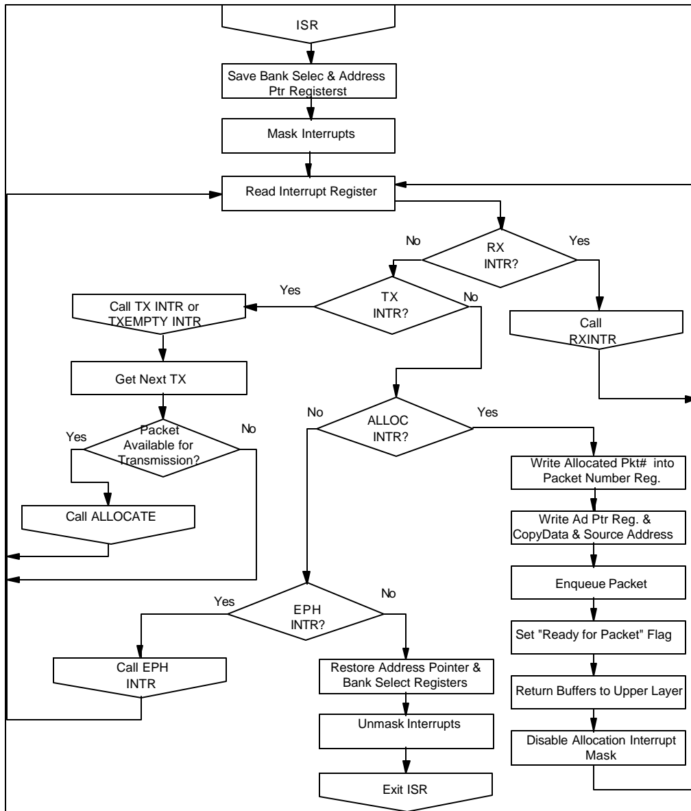
FIGURE 13 - INTERRUPT SERVICE ROUTINE
