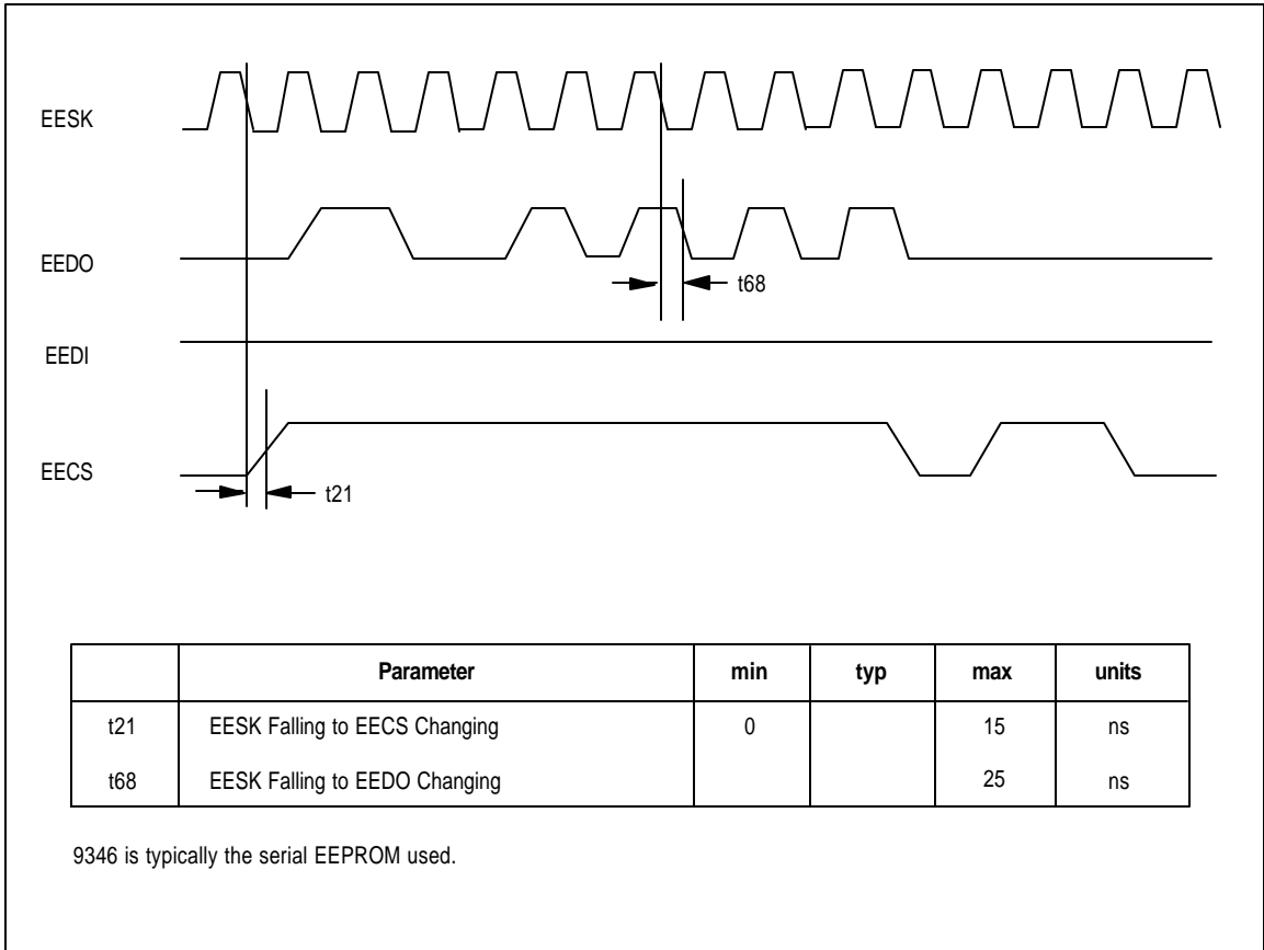
FIGURE 30 - EEPROM READ
