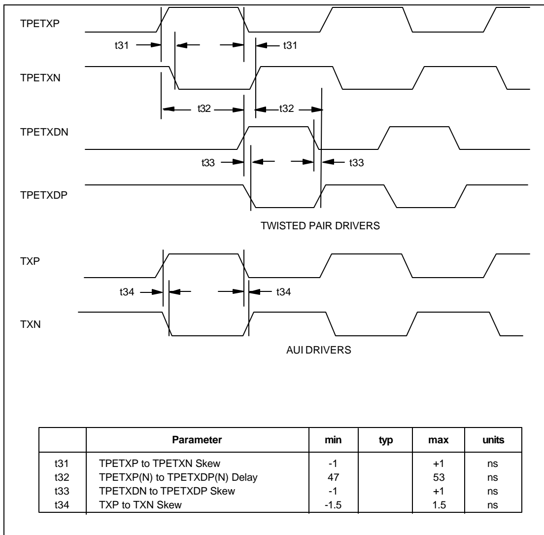
FIGURE 34 - DIFFERENTIAL OUTPUT SIGNAL TIMING (10BASE-T AND AUI)
