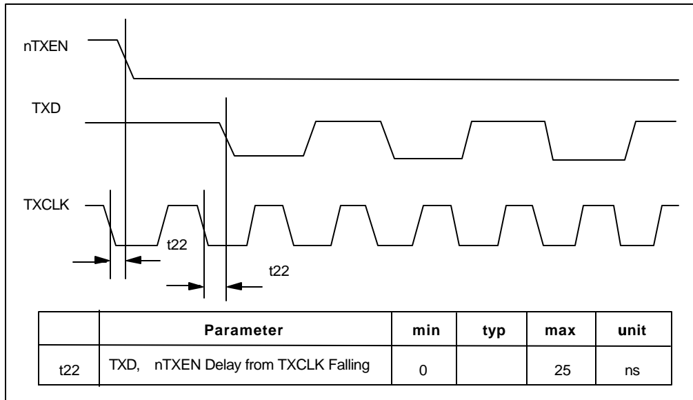
FIGURE 32 - EXTERNAL ENDEC INTERFACE - START OF TRANSMIT
