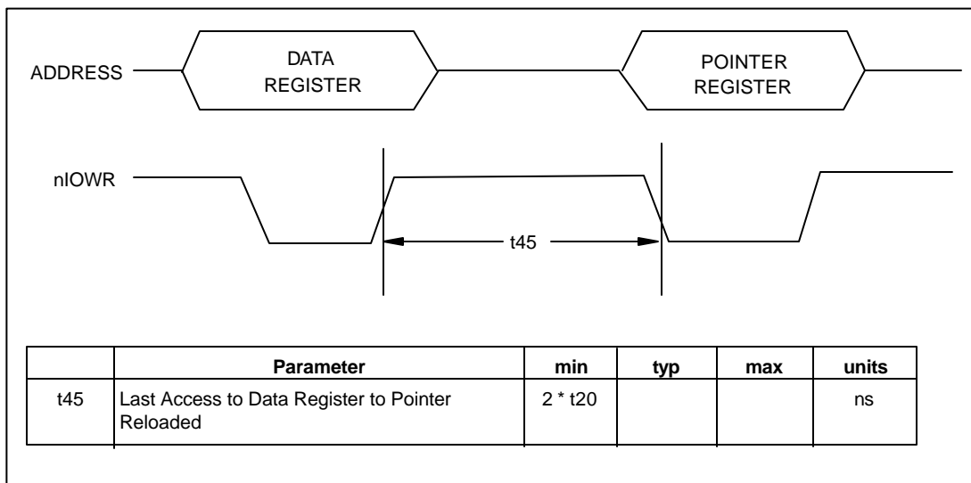
FIGURE 41 - MEMORY WRITE TIMING
