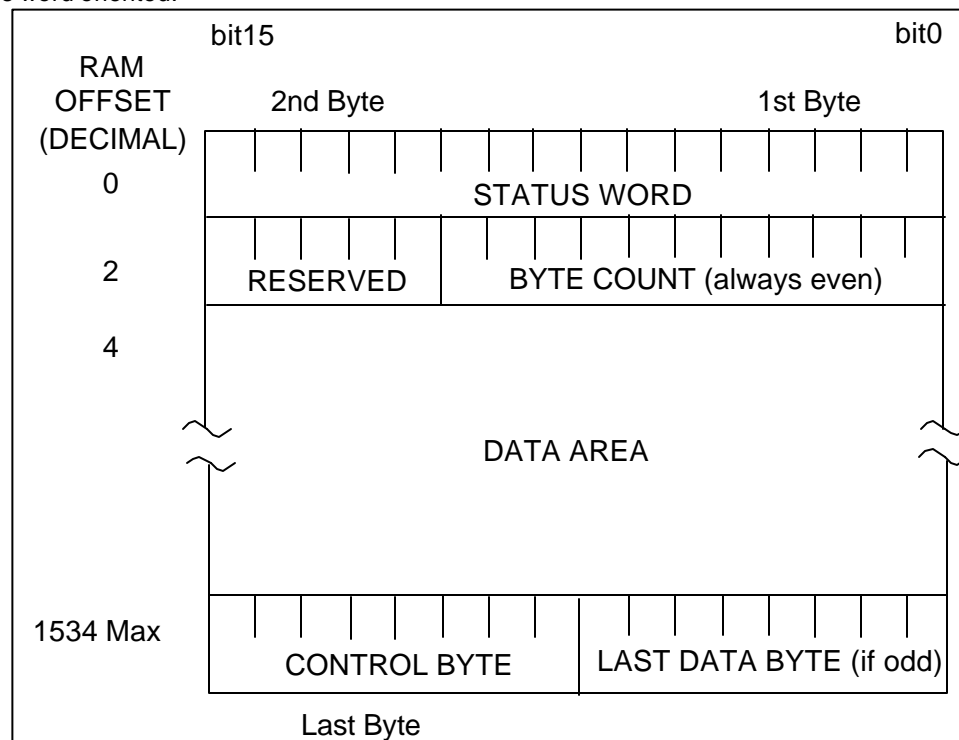
FIGURE 10 – DATA PACKET FORMAT
