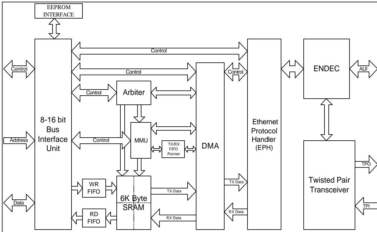
FIGURE 8 – LAN91C96I INTERNAL BLOCK DIAGRAM WITH DATA PATH
