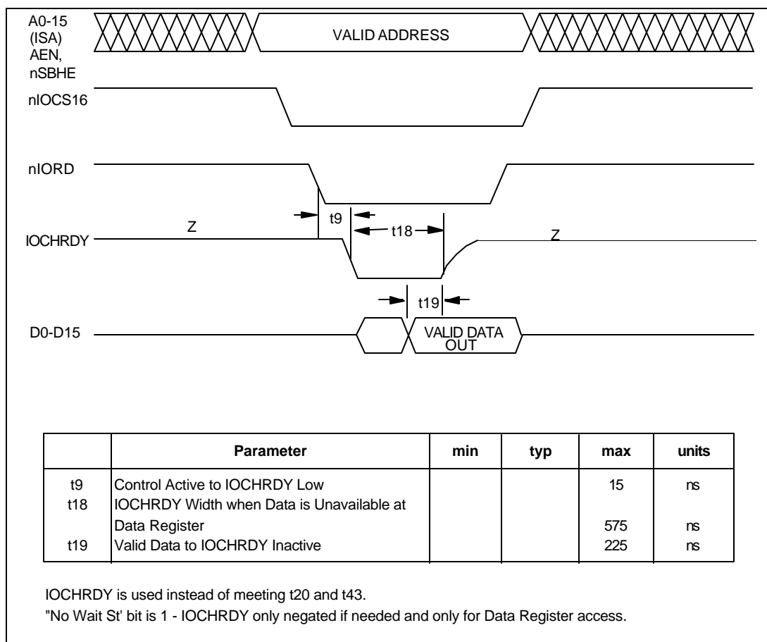
FIGURE 24 - DATA REGISTER SPECIAL READ ACCESS
