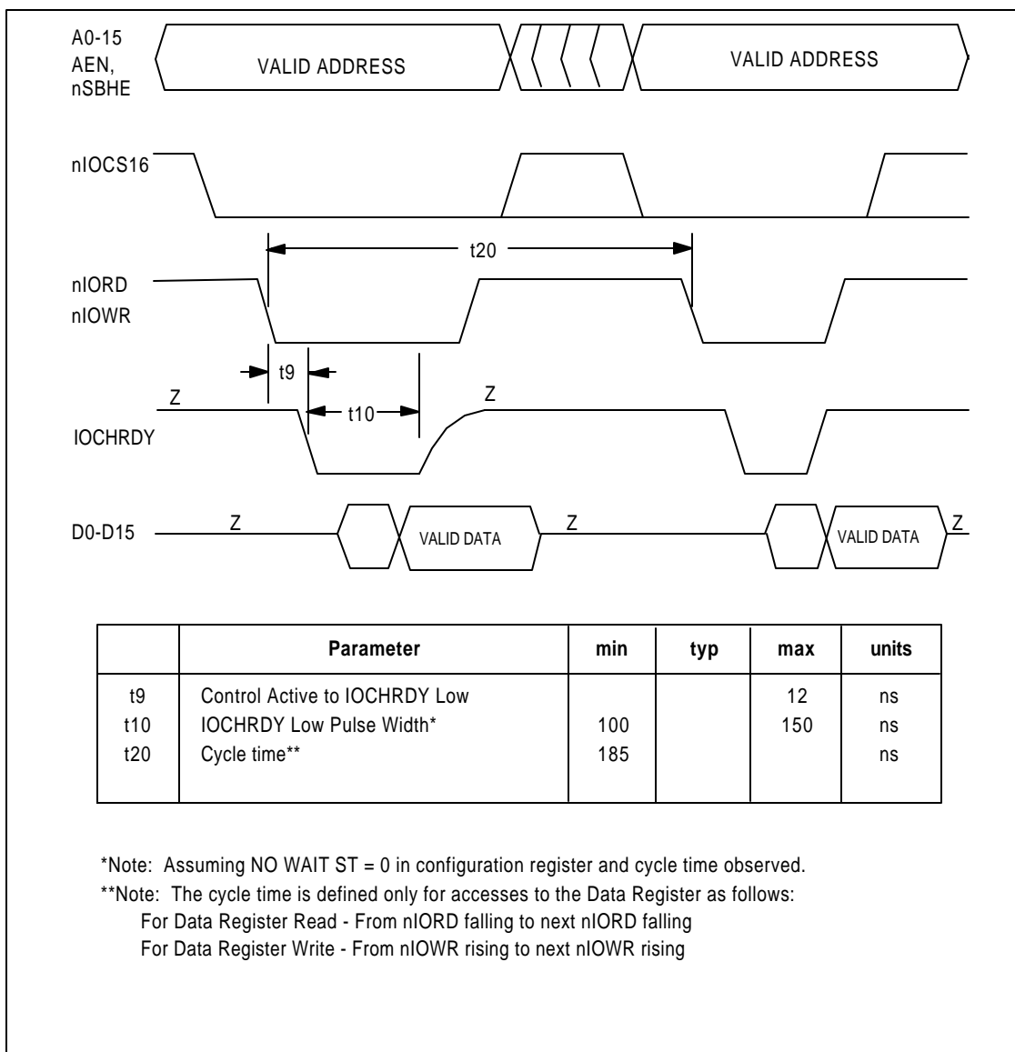
FIGURE 23 - LOCAL BUS CONSECUTIVE READ AND WRITE CYCLES
