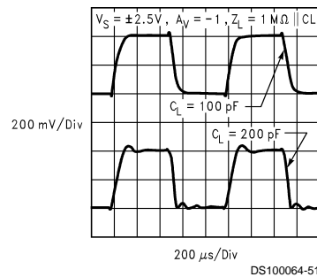
Small Signal Step Response ( A_V = -1 ) ( C_L = 1M\Omega \parallel 100 pF, 200 pF )
