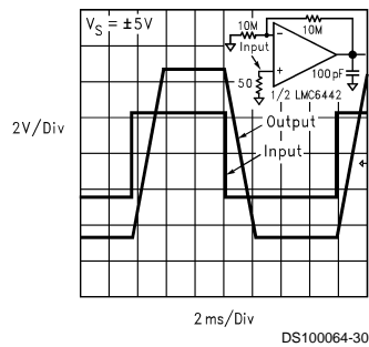
Large Signal Step Response ( A_V = +2 ) ( C_L = 100 pF )
