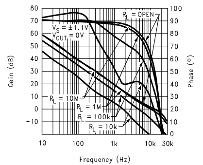
Open Loop Gain/Phase vs Frequency
