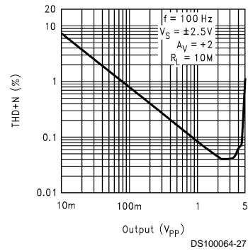
THD+N vs Amplitude
