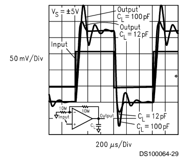
Small Signal Step Response ( A_V = +2 ) ( C_L = 12 pF, 100 pF )
