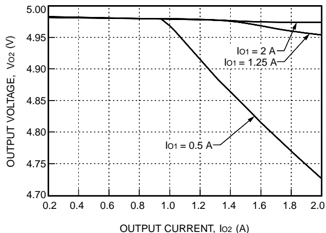
Figure 7. LW016FA Load Regulation ( V_{O2} )
