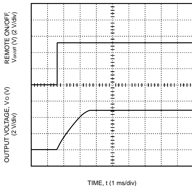
Figure 6. LW016FA Typical Output Voltage Start-Up When Signal Applied to Remote On/Off
