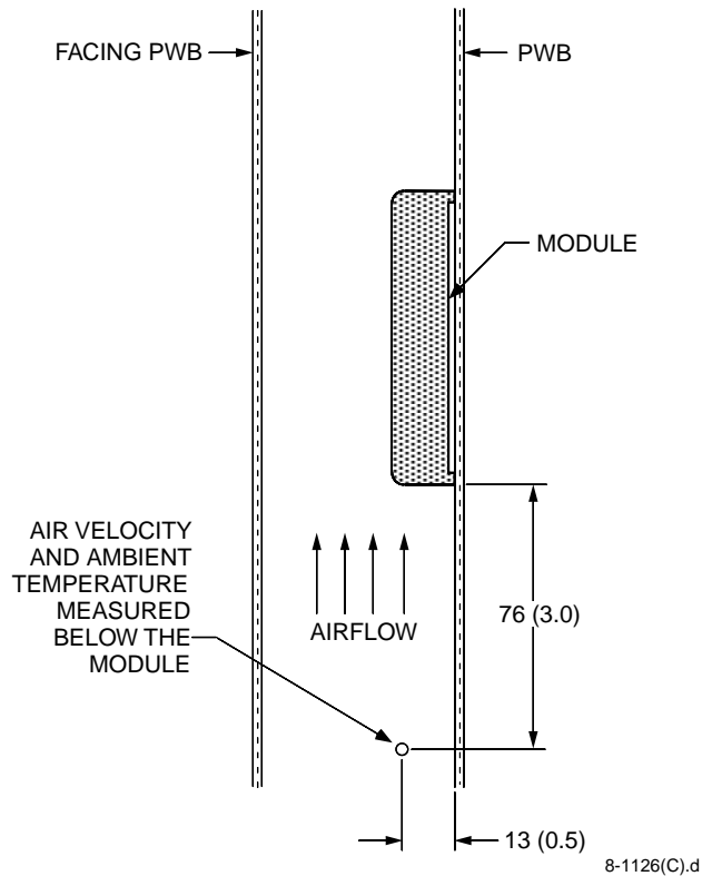
Figure 15. Experimental Test Setup
