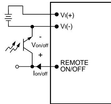
Figure 11. Remote On/Off Implementation
