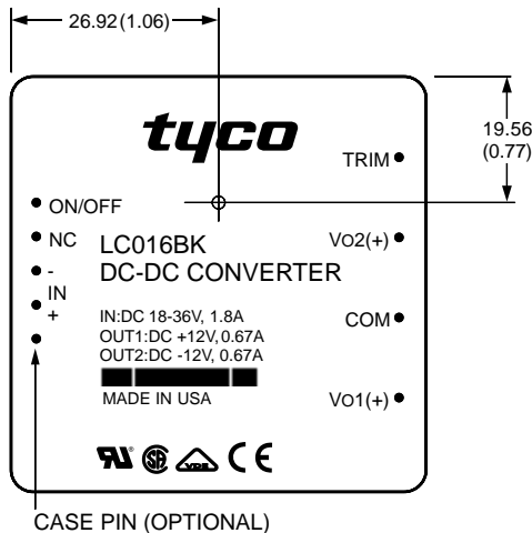
Figure 12. Case Temperature Measurement Location
