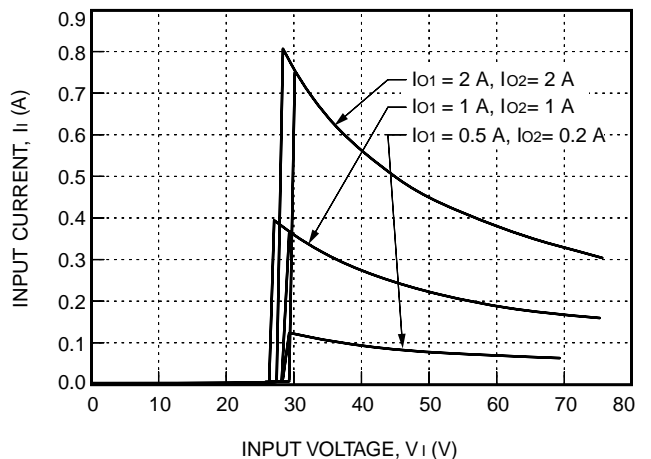
Figure 1. LW016AF and LW016FA Typical Input Characteristics
