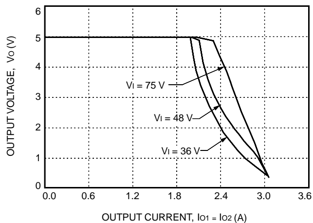
Figure 2. LW016AF and LW016FA Typical Output Characteristics
