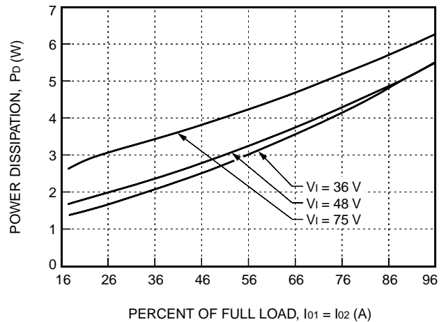
Figure 13. LW016FA Power Dissipation vs. Output Current
