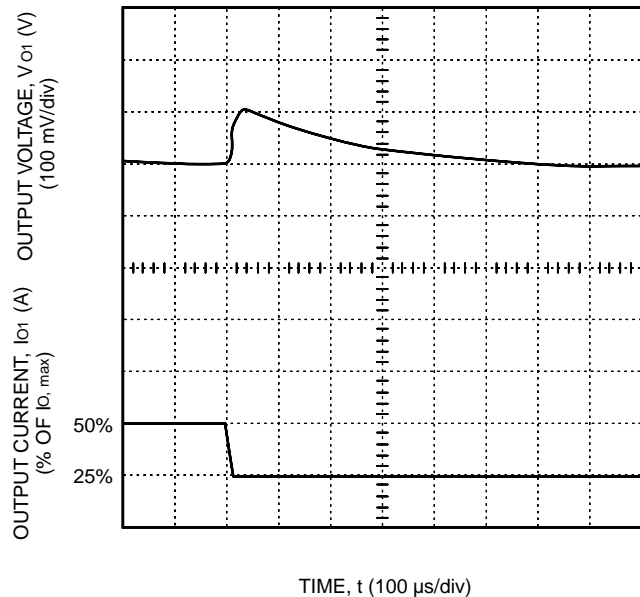
Figure 5. LW016AF and LW016FA Typical Output Voltage for a Step Load Change from 50% to 25%
