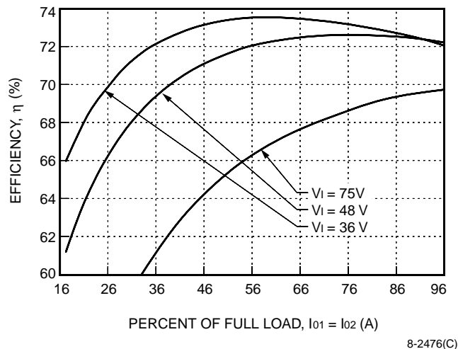
Figure 3. LW016FA Typical Converter Efficiency vs. Output Current
