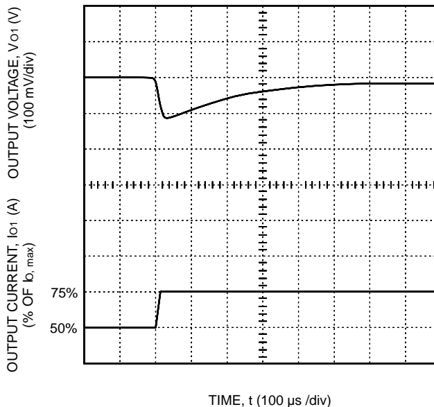
Figure 4. LW016AF and LW016FA Typical Output Voltage for a Step Load Change from 50% to 75%
