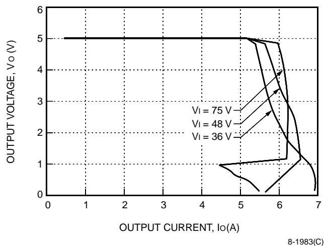
Figure 4. LW025A Typical Output Characteristics
