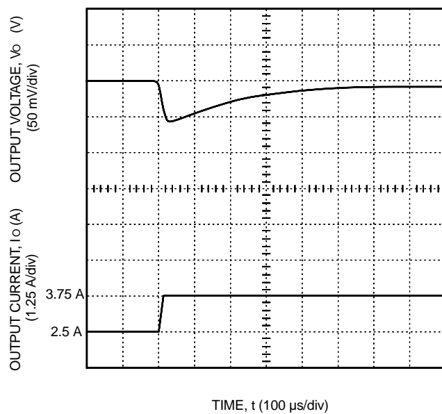
Figure 8. LW025A, F Typical Output Voltage for a Step Load Change from 50% to 75%
