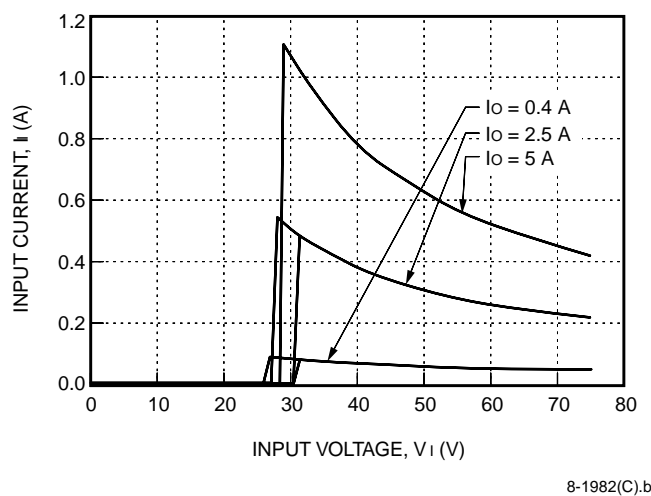
Figure 2. LW025A Typical Input Characteristics
