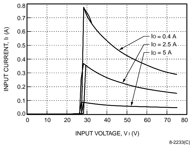
Figure 1. LW025F Typical Input Characteristics
