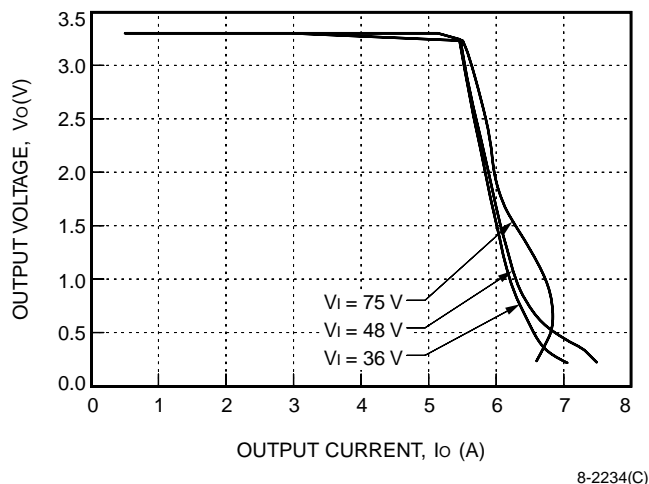
Figure 3. LW025F Typical Output Characteristics
