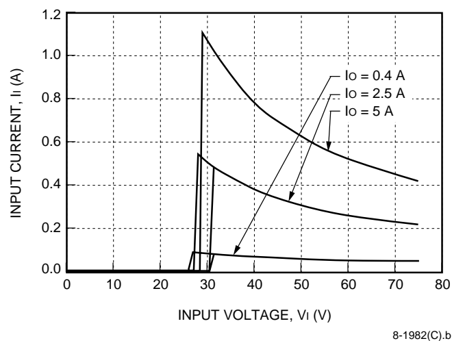
Figure 2. LUW025A Typical Input Characteristics
