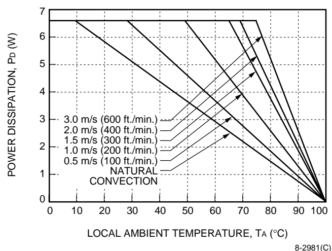
Figure 22. LUW025A Power Derating vs. Local Ambient Temperature and Air Velocity; Orientation 1
