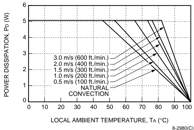
Figure 21. LUW025F Power Derating vs. Local Ambient Temperature and Air Velocity; Orientation 1 (Preliminary)
