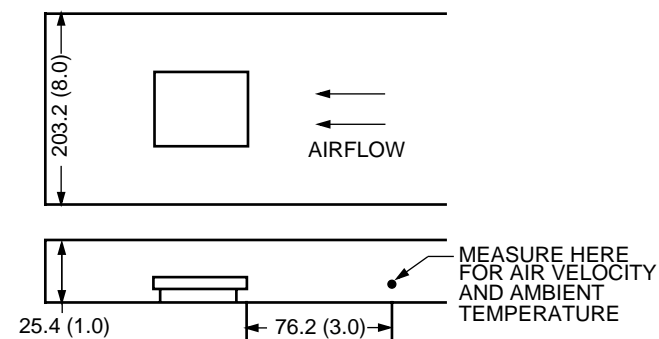
Figure 16. Thermal Test Setup
