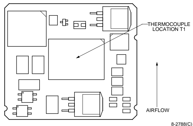
Figure 17. T_a Temperature Measurement Location; Top View; Orientation 1
