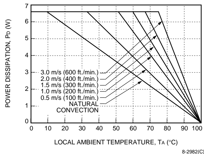
Figure 24. LUW025A Power Derating vs. Local Ambient Temperature and Air Velocity; Orientation 2
