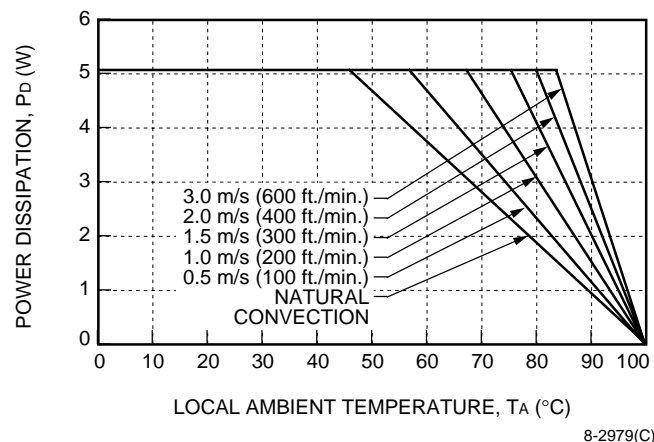
Figure 23. LUW025F Power Derating vs. Local Ambient Temperature and Air Velocity; Orientation 2 (Preliminary)
