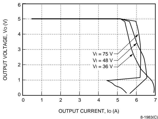
Figure 4. LUW025A Typical Output Characteristics
