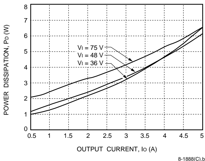
Figure 20. LUW025A Power Dissipation vs. Output Current, T_a = 25\text{ }^{\circ}\text{C} ; Either Orientation
