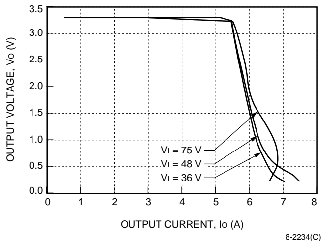
Figure 3. LUW025F Typical Output Characteristics
