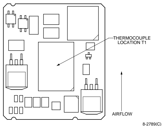
Figure 18. T_a Temperature Measurement Location; Top View; Orientation 2
