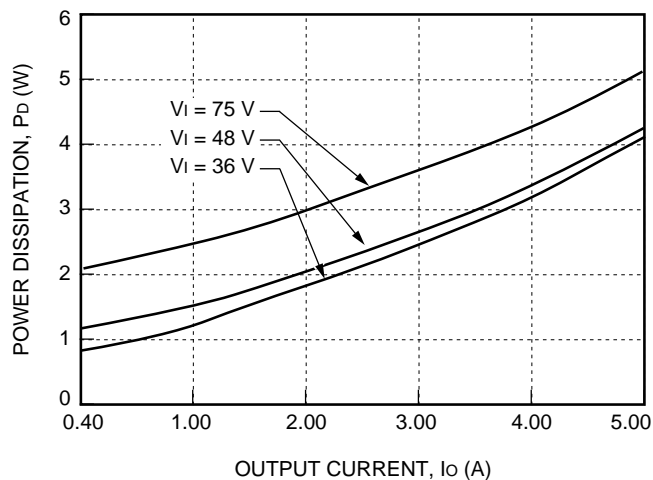
Figure 19. LUW025F Power Dissipation vs. Output Current, T_a = 25\text{ }^{\circ}\text{C} ; Either Orientation
