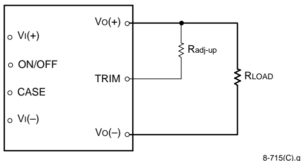
Figure 15. Circuit Configuration to Increase Output Voltage
