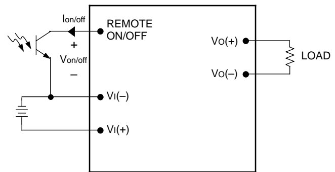
Figure 13. Remote On/Off Implementation
