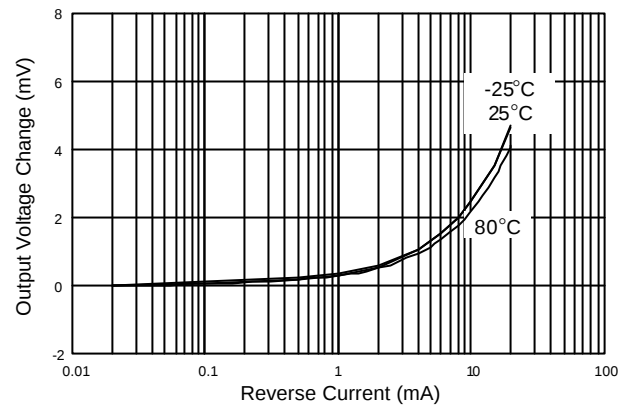
Fig. 2 Reverse Characteristics
