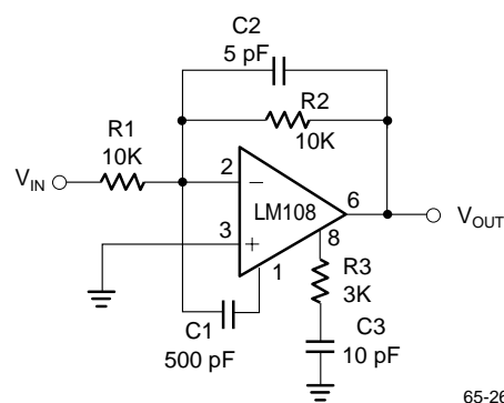
Figure 6. Feedforward Compensation
