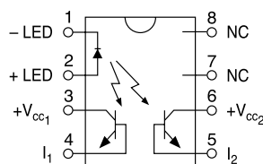
LOC112 Pinout
