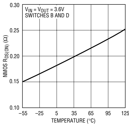
NMOS R_{DS(ON)}
