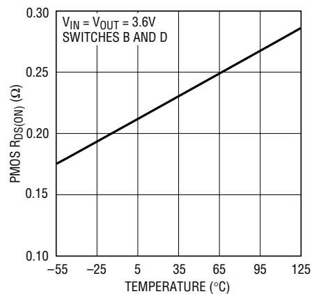
PMOS R_{DS(ON)}
