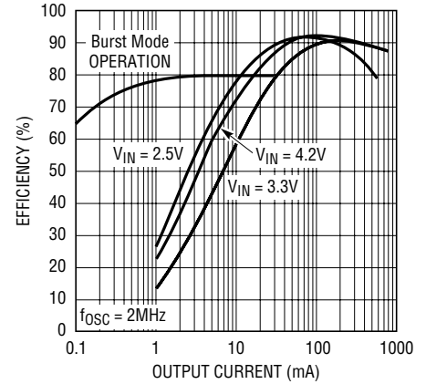
Li-Ion to 3.3V Efficiency ( f_{OSC} = 2MHz )
