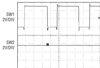
Switch Pins in Buck Mode
