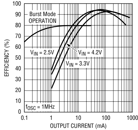
Li-Ion to 3.3V Efficiency ( f_{OSC} = 1MHz )
