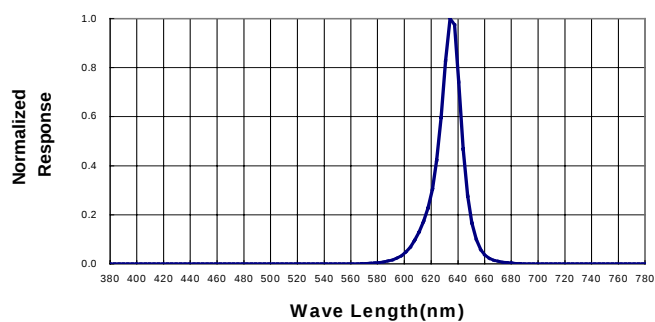
Spectral Radiance (Peak @ 636nm)
