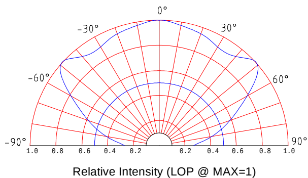
Beam Pattern
