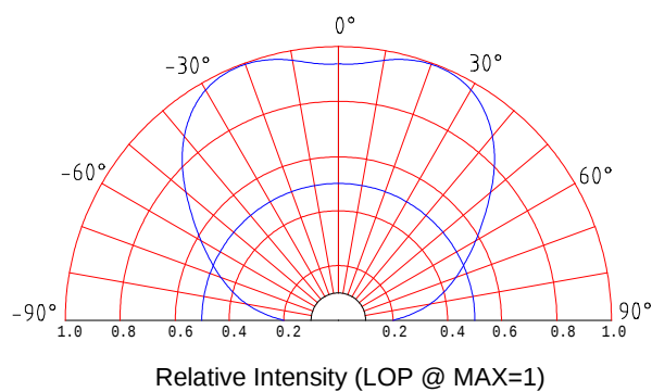
Beam Pattern
