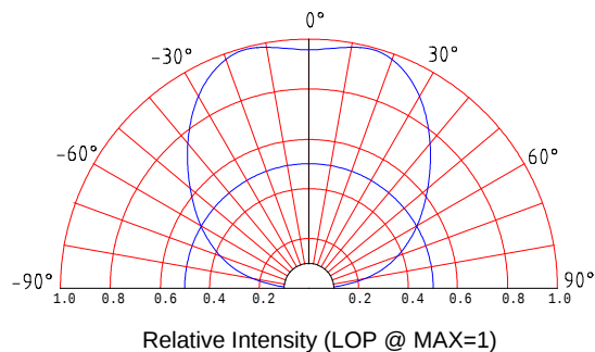
Beam Pattern
