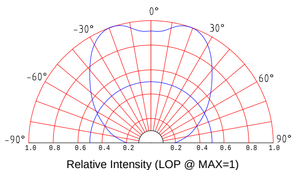
Beam Pattern
