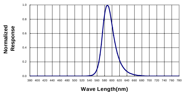
Spectral Radiance ( Peak @ 588 nm)
