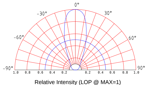
Beam Patter
