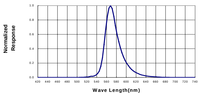
Spectral Radiance (Peak @ 568nm)
