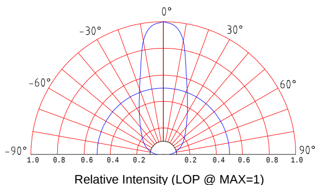
Beam Pattern
