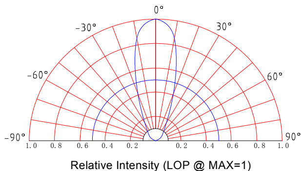
Beam Patter
