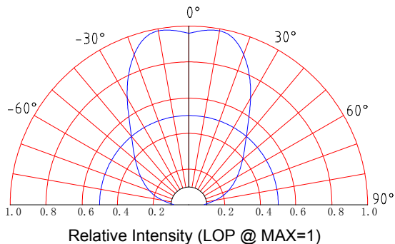
Beam Pattern
